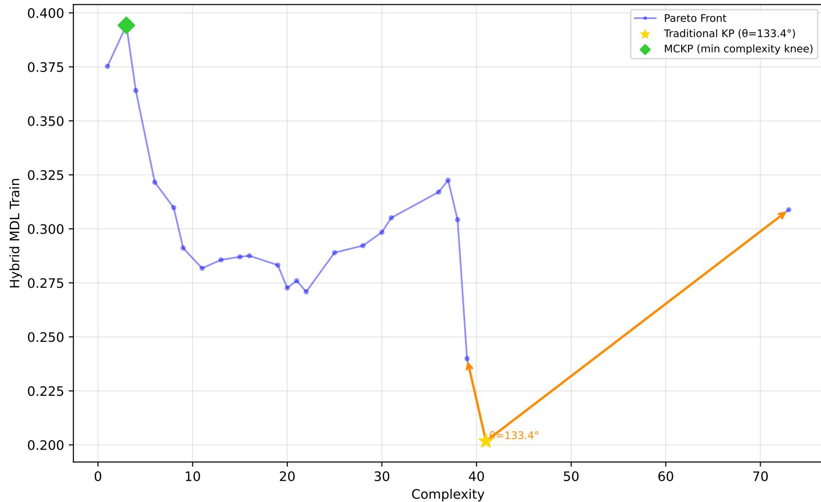
637_fri_c1_500_50 - Run 23 - SVP - Hybrid MDL Train \lambda_1=0.10, \lambda_2=0.00, \lambda_3=0.20 | Difficulty: 1.00 | Method: hmr
