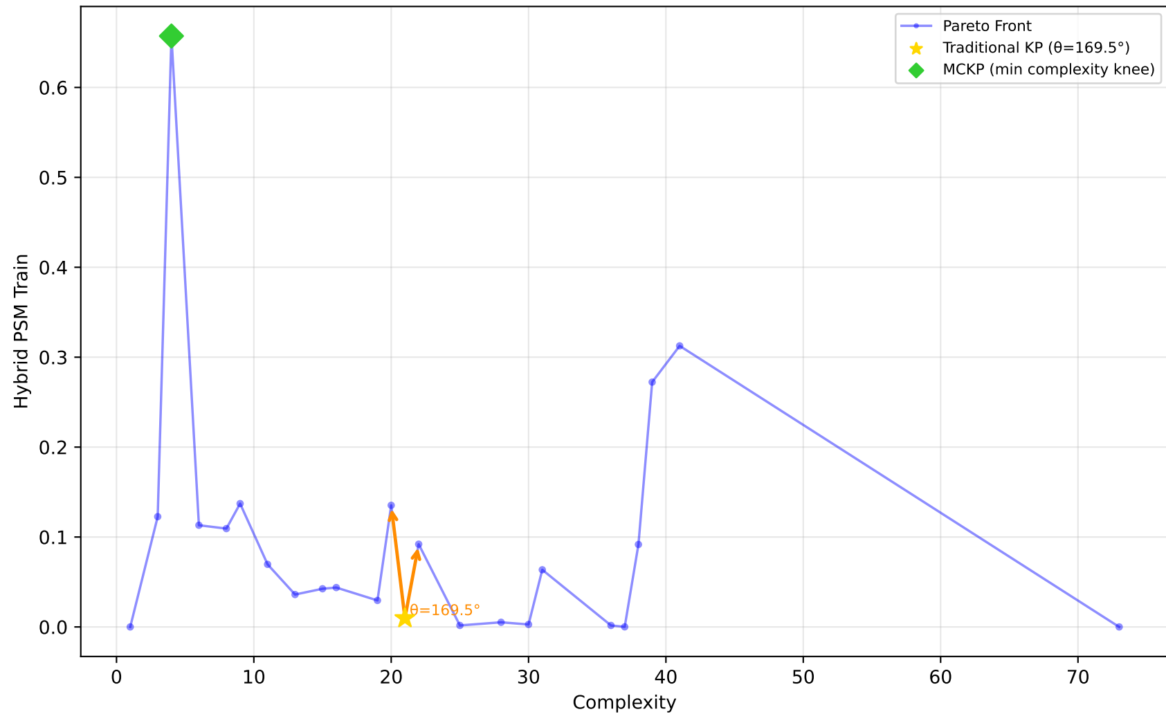
637_fri_c1_500_50 - Run 23 - SVP - Hybrid PSM Train \lambda_1=0.00, \lambda_2=0.00, \lambda_3=0.00 | Difficulty: 1.00 | Method: hmr
