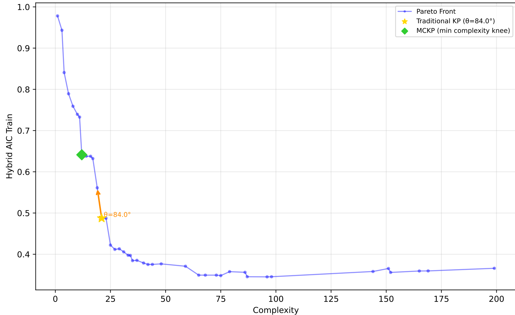
637_fri_c1_500_50 - Run 24 - MVP - Hybrid AIC Train \lambda_1=0.00, \lambda_2=0.50, \lambda_3=0.00 | Difficulty: 1.00 | Method: hmr
