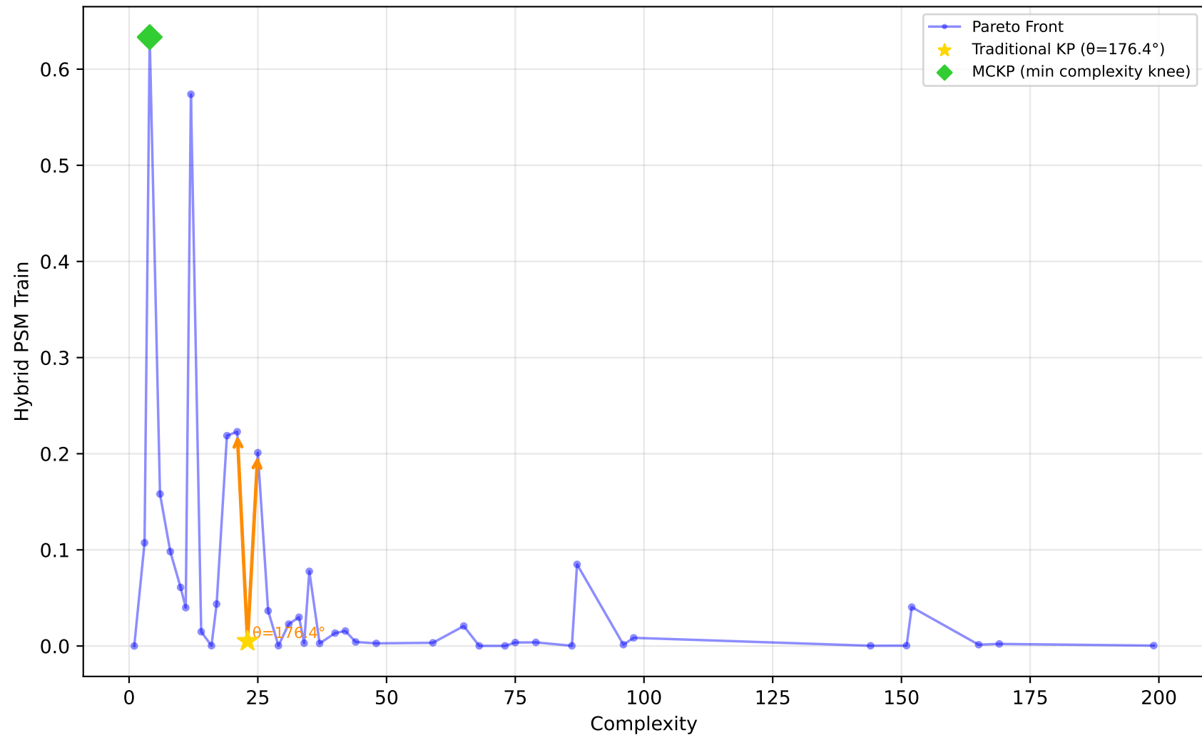
637_fri_c1_500_50 - Run 24 - MVP - Hybrid PSM Train \lambda_1=0.00, \bar{\lambda}_2=0.50, \bar{\lambda}_3=0.00 | Difficulty: 1.00 | Method: hmr
