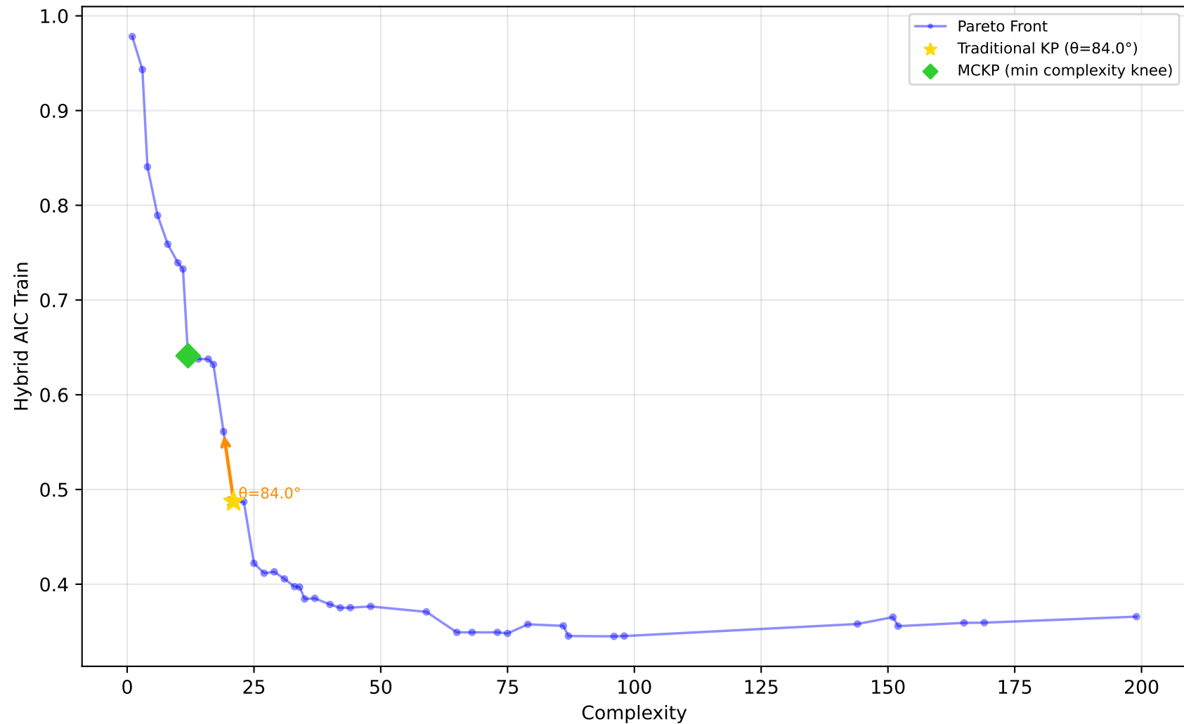
637_fri_c1_500_50 - Run 24 - SVP - Hybrid AIC Train \lambda_1=0.00, \lambda_2=0.00, \lambda_3=0.00 | Difficulty: 1.00 | Method: hmr
