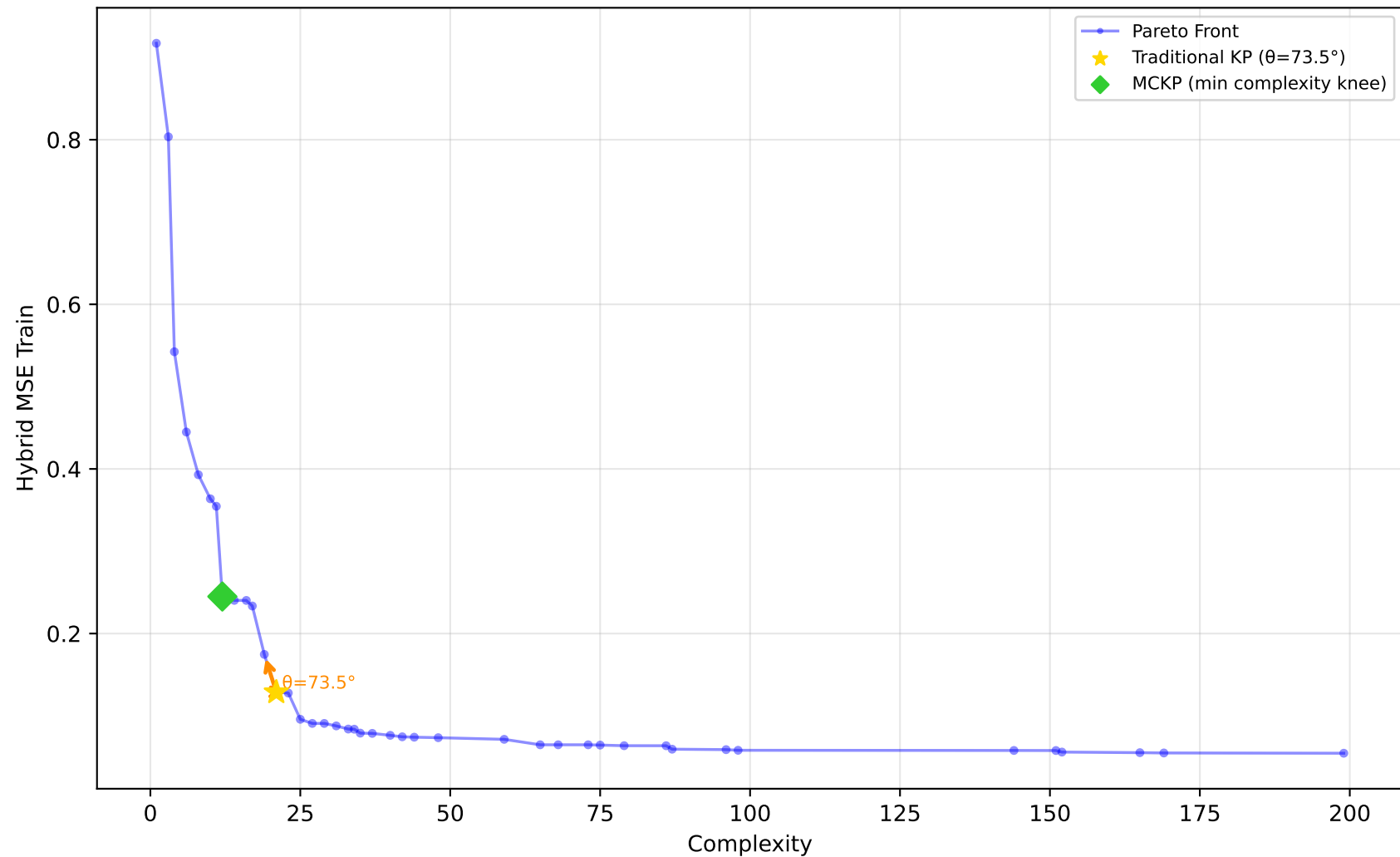
637_fri_c1_500_50 - Run 24 - SVP - Hybrid MSE Train \lambda_1=0.00, \lambda_2=0.00, \lambda_3=0.00 | Difficulty: 1.00 | Method: hmr
