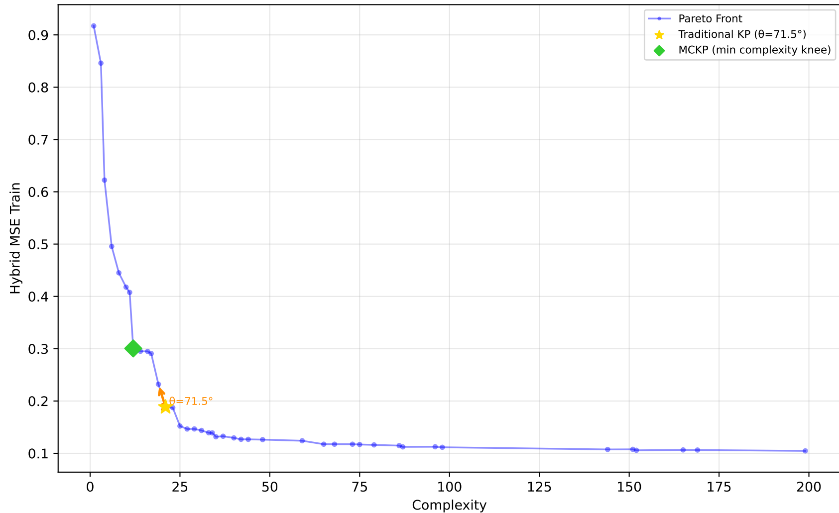
637_fri_c1_500_50 - Run 24 - SVP - Hybrid MSE Train \lambda_1=0.10, \lambda_2=0.00, \lambda_3=0.20 | Difficulty: 1.00 | Method: hmr
