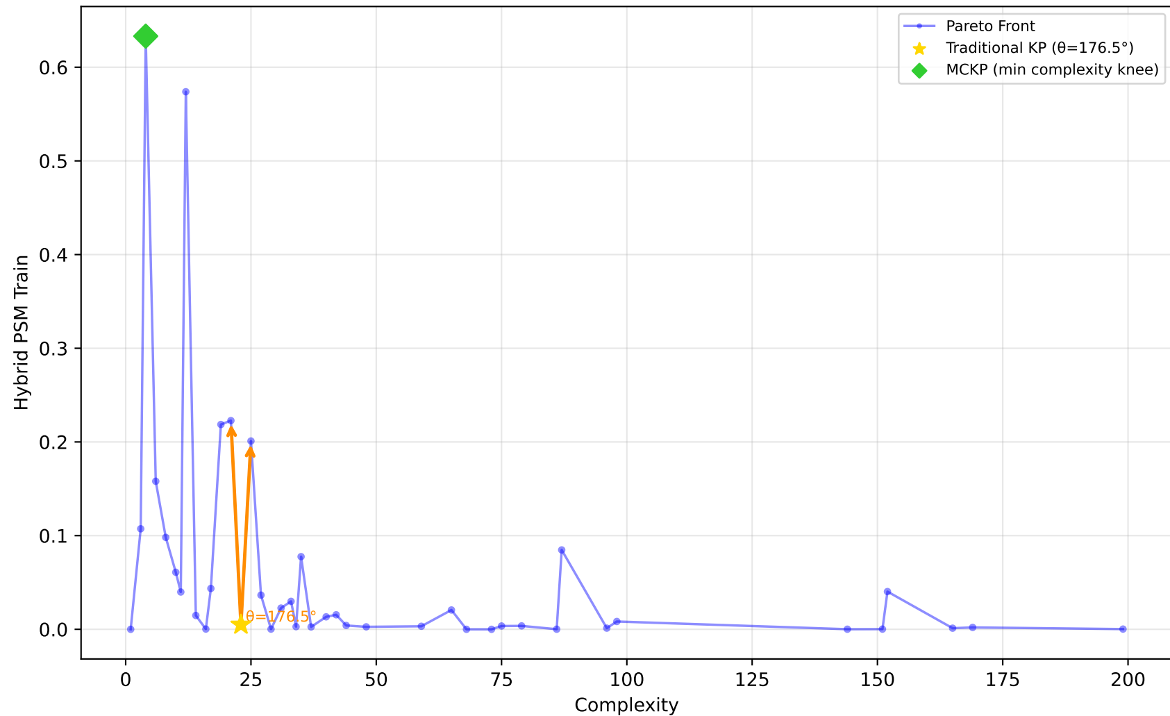
637_fri_c1_500_50 - Run 24 - SVP - Hybrid PSM Train \lambda_1=0.00, \lambda_2=0.00, \lambda_3=0.00 | Difficulty: 1.00 | Method: hmr
