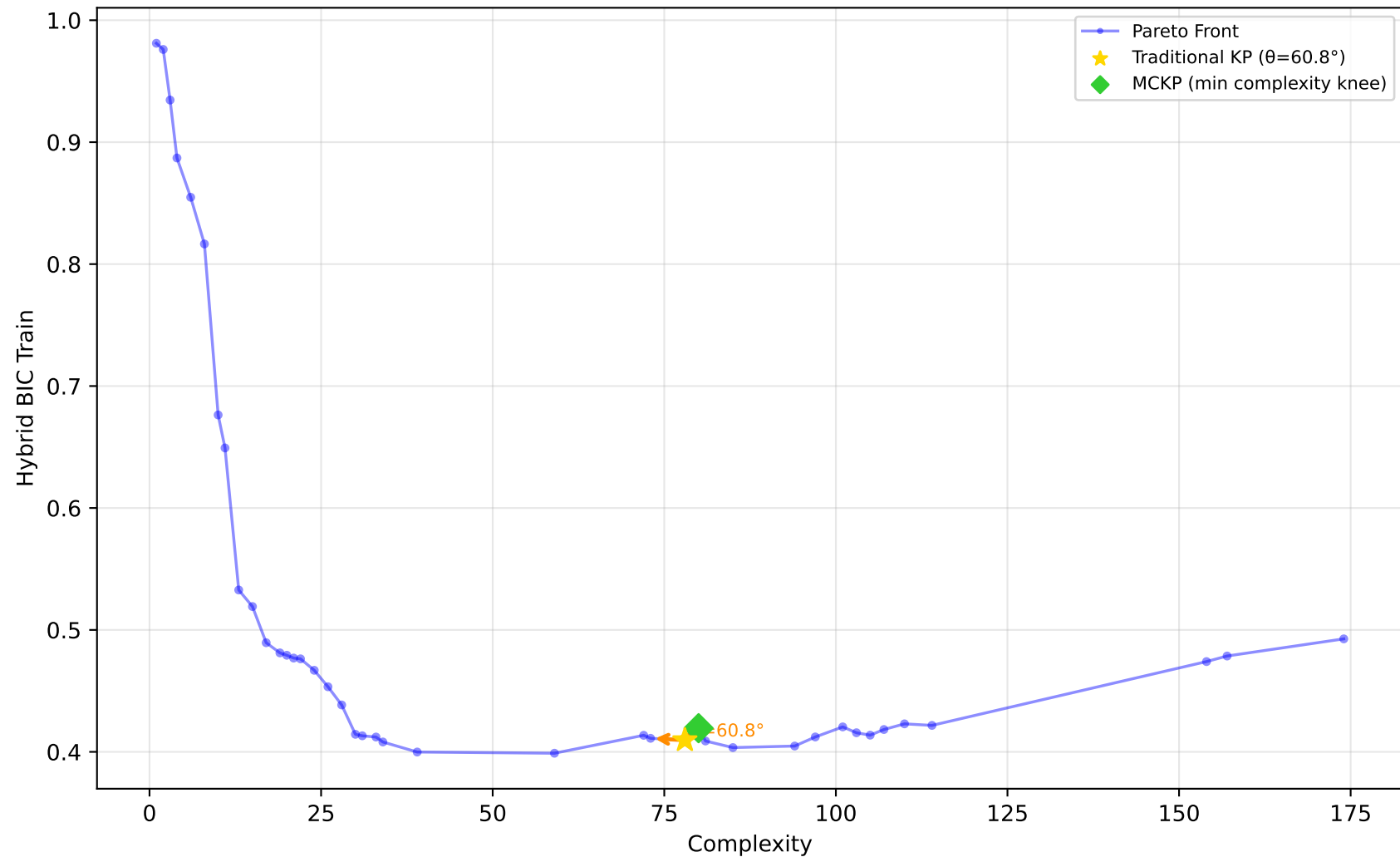
637_fri_c1_500_50 - Run 25 - MVP - Hybrid BIC Train \lambda_1=0.00, \lambda_2=0.50, \lambda_3=0.00 | Difficulty: 1.00 | Method: hmr
