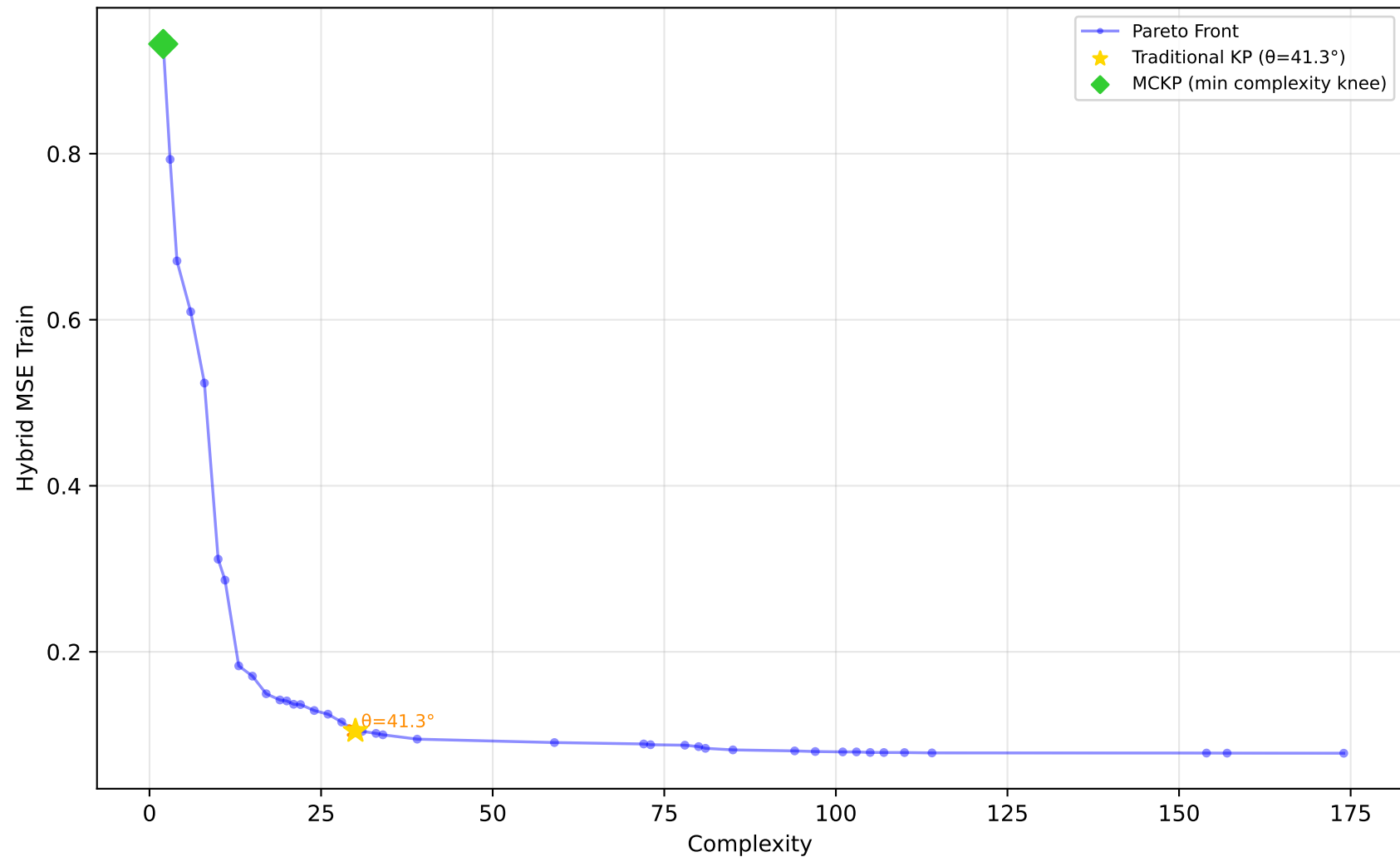
637_fri_c1_500_50 - Run 25 - SVP - Hybrid MSE Train \lambda_1=0.00, \lambda_2=0.00, \lambda_3=0.00 | Difficulty: 1.00 | Method: hmr
