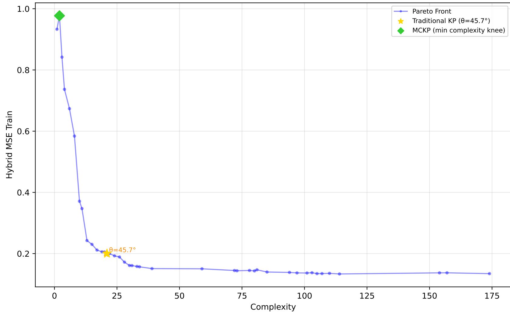
637_fri_c1_500_50 - Run 25 - SVP - Hybrid MSE Train \lambda_1=0.10, \lambda_2=0.00, \lambda_3=0.20 | Difficulty: 1.00 | Method: hmr
