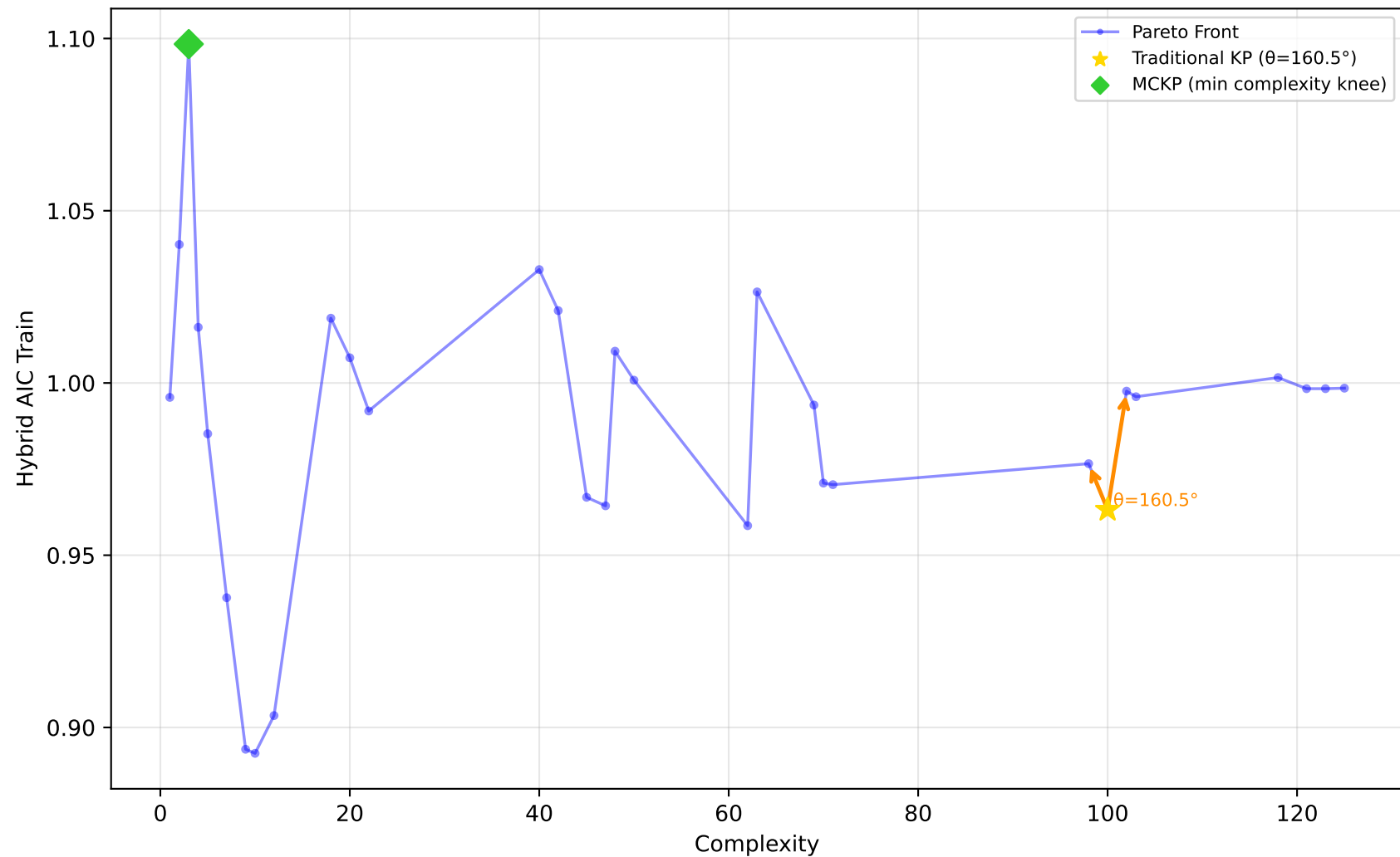
637_fri_c1_500_50 - Run 26 - MVP - Hybrid AIC Train \lambda_1=0.10, \lambda_2=0.00, \lambda_3=1.00 | Difficulty: 1.00 | Method: hmr
