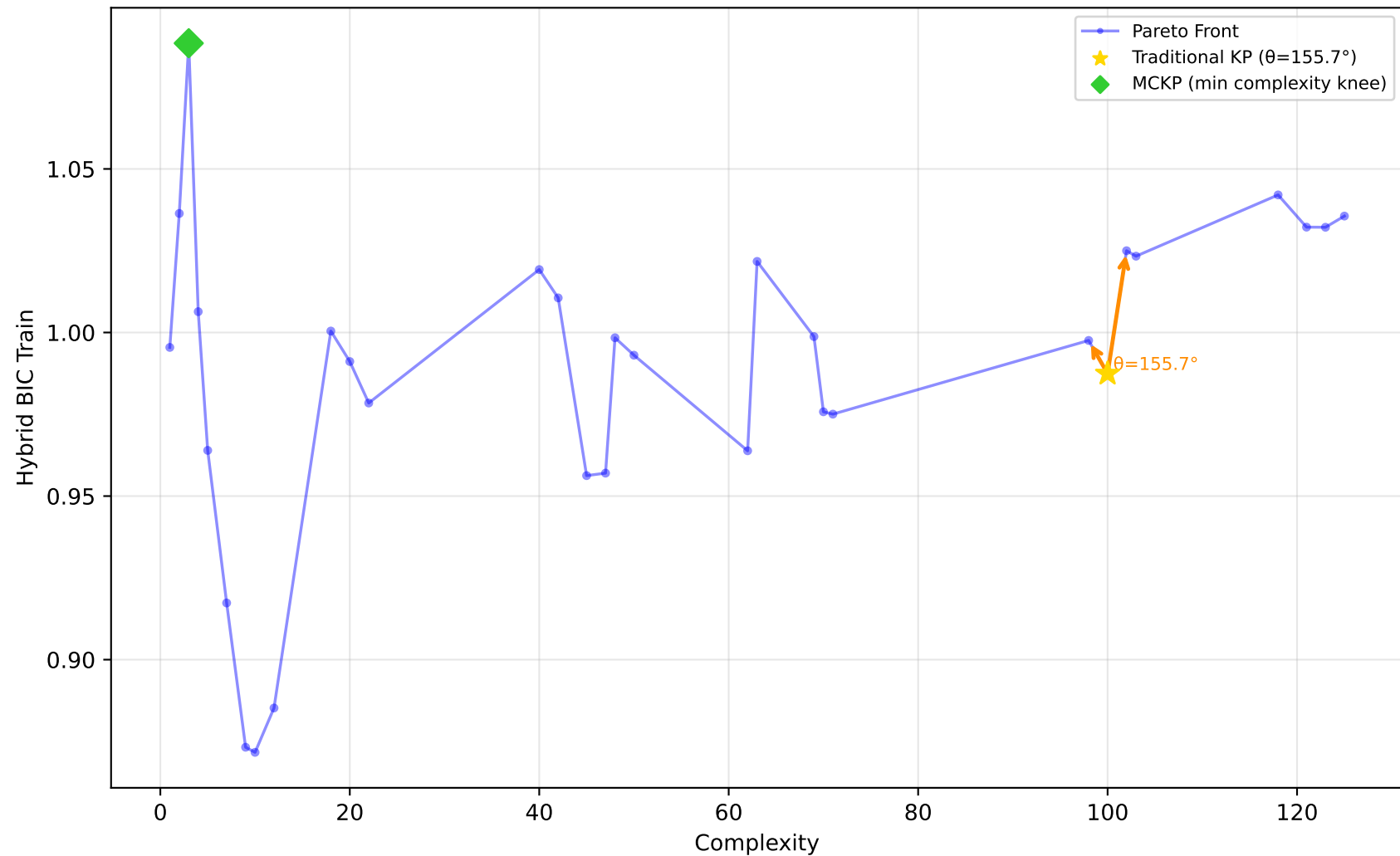
637_fri_c1_500_50 - Run 26 - MVP - Hybrid BIC Train \lambda_1=0.10, \lambda_2=0.00, \lambda_3=1.00 | Difficulty: 1.00 | Method: hmr
