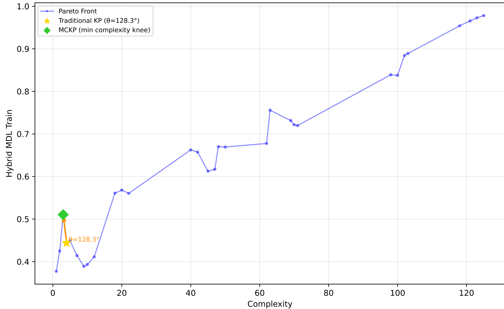
637_fri_c1_500_50 - Run 26 - MVP - Hybrid MDL Train \lambda_1=0.10, \bar{\lambda}_2=0.00, \bar{\lambda}_3=1.00 | Difficulty: 1.00 | Method: hmr
