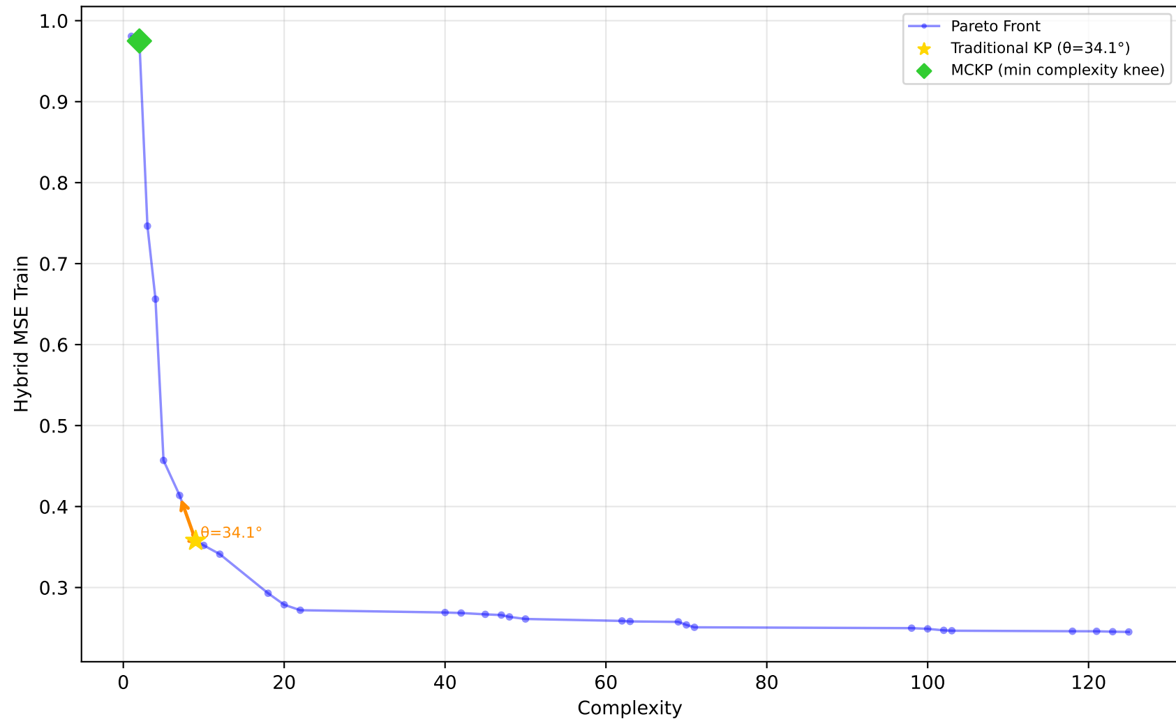
637_fri_c1_500_50 - Run 26 - MVP - Hybrid MSE Train \lambda_1=0.00, \bar{\lambda}_2=0.50, \lambda_3=0.00 | Difficulty: 1.00 | Method: hmr
