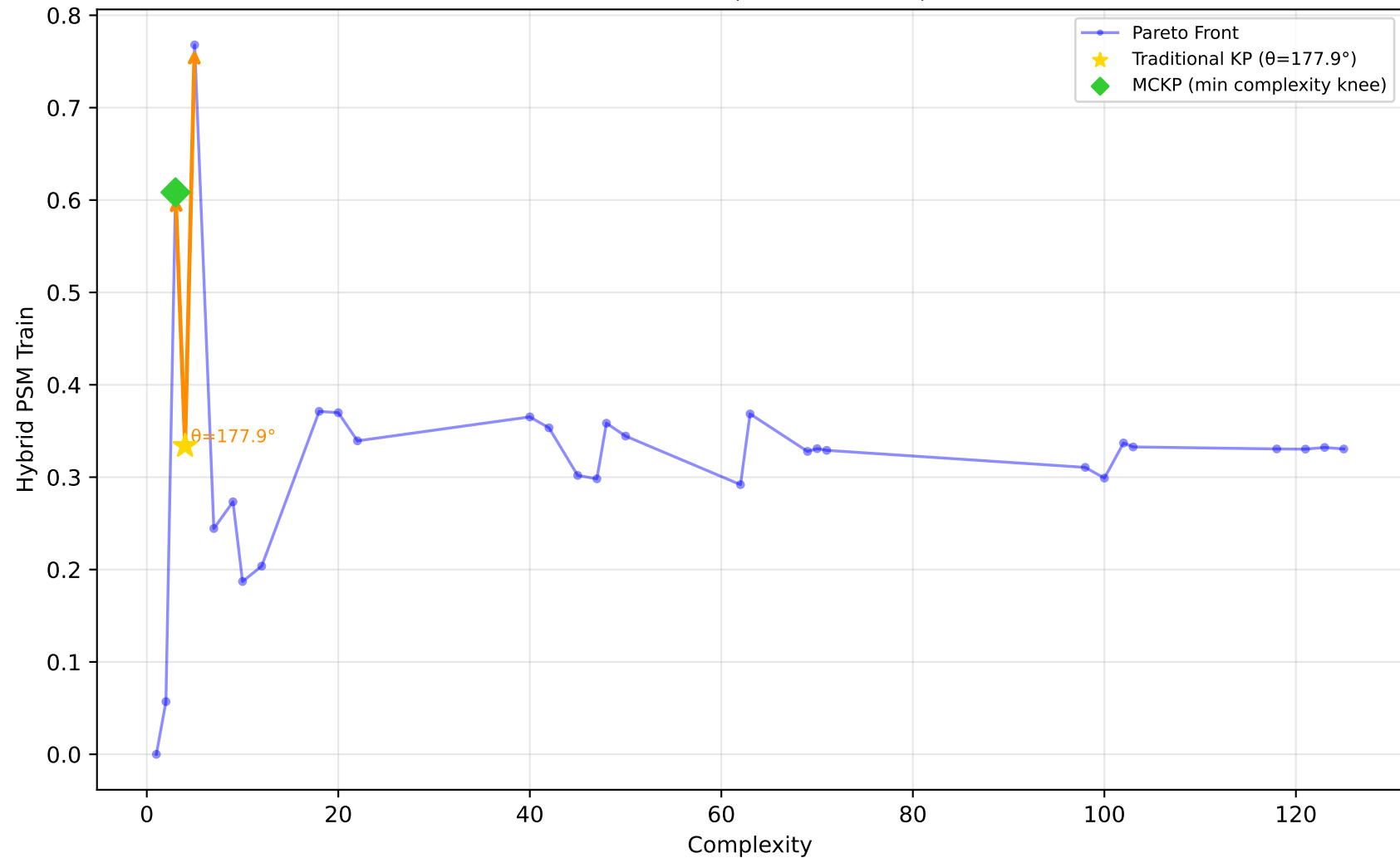
637_fri_c1_500_50 - Run 26 - MVP - Hybrid PSM Train \lambda_1=0.10, \bar{\lambda}_2=0.00, \bar{\lambda}_3=1.00 | Difficulty: 1.00 | Method: hmr
