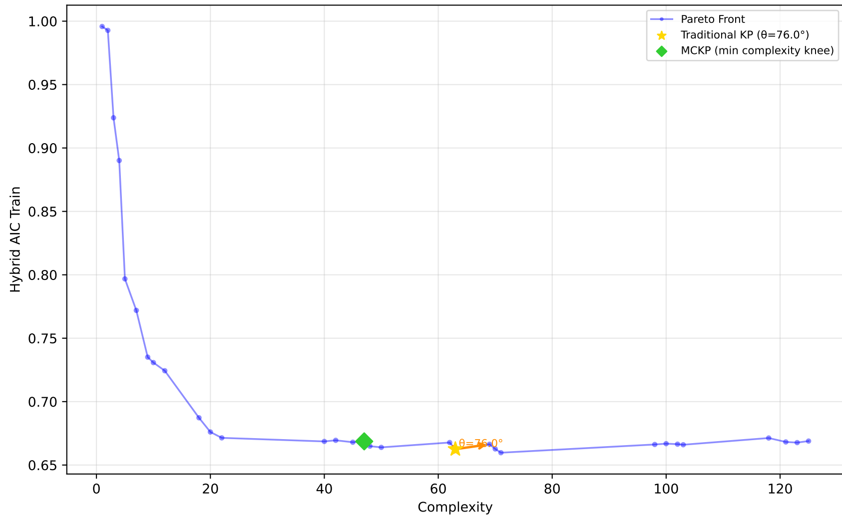
637_fri_c1_500_50 - Run 26 - SVP - Hybrid AIC Train \lambda_1=0.00, \lambda_2=0.00, \lambda_3=0.00 | Difficulty: 1.00 | Method: hmr
