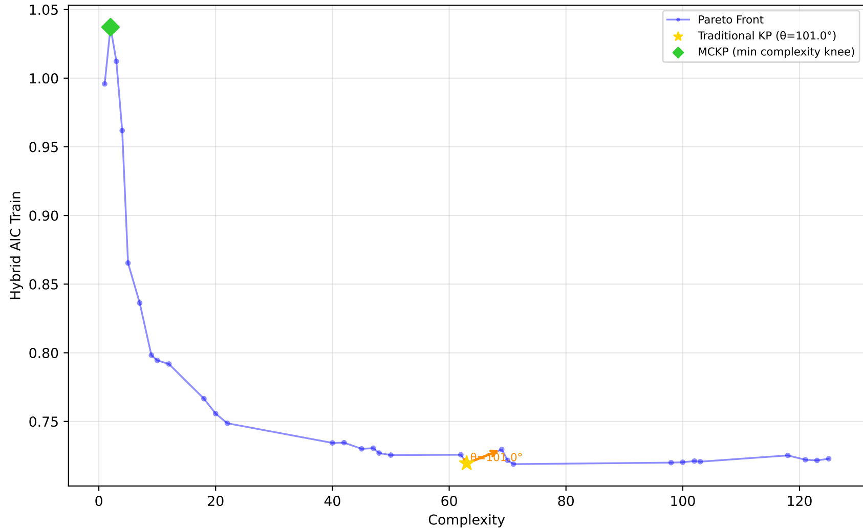
637_fri_c1_500_50 - Run 26 - SVP - Hybrid AIC Train \lambda_1=0.10 , \lambda_2=0.00 , \lambda_3=0.20 | Difficulty: 1.00 | Method: hmr
