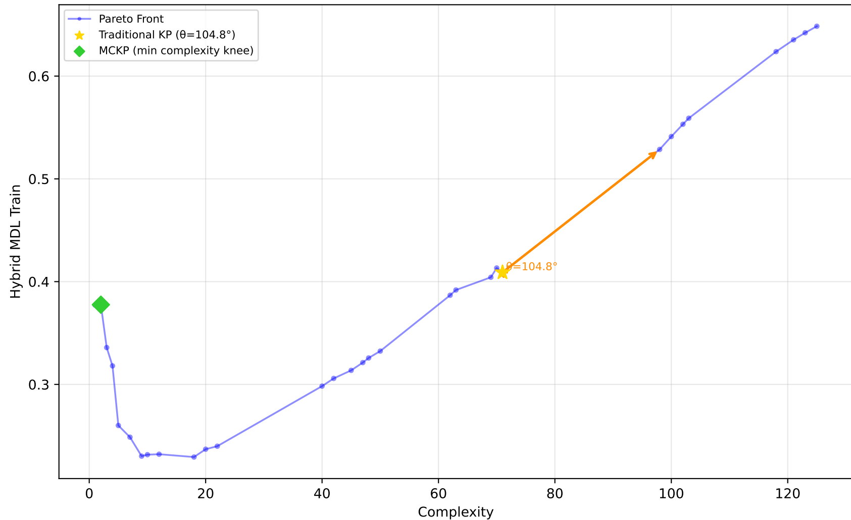
637_fri_c1_500_50 - Run 26 - SVP - Hybrid MDL Train \lambda_1=0.00, \lambda_2=0.00, \lambda_3=0.00 | Difficulty: 1.00 | Method: hmr
