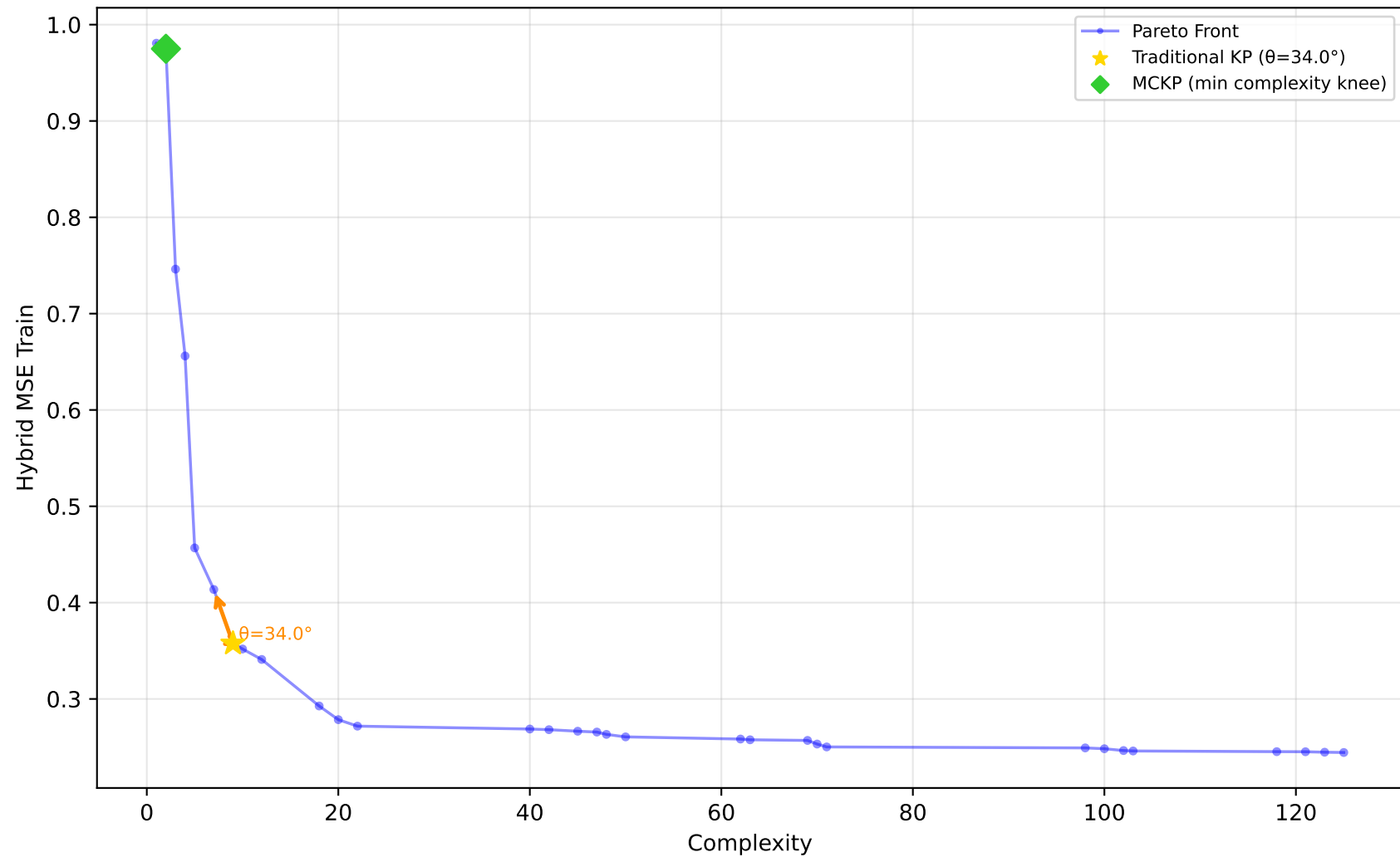
637_fri_c1_500_50 - Run 26 - SVP - Hybrid MSE Train \lambda_1=0.00, \lambda_2=0.00, \lambda_3=0.00 | Difficulty: 1.00 | Method: hmr
