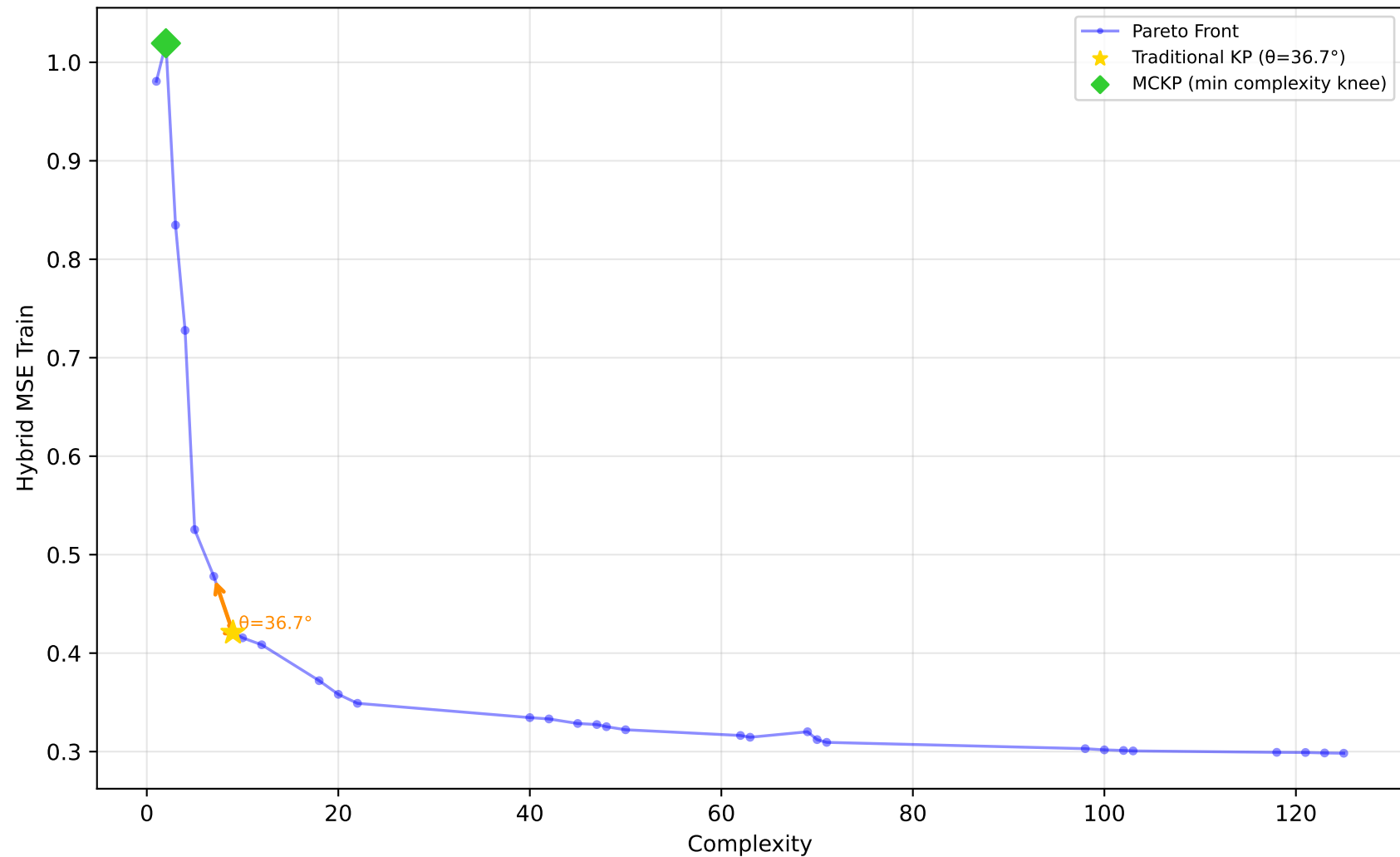
637_fri_c1_500_50 - Run 26 - SVP - Hybrid MSE Train \lambda_1=0.10, \lambda_2=0.00, \lambda_3=0.20 | Difficulty: 1.00 | Method: hmr
