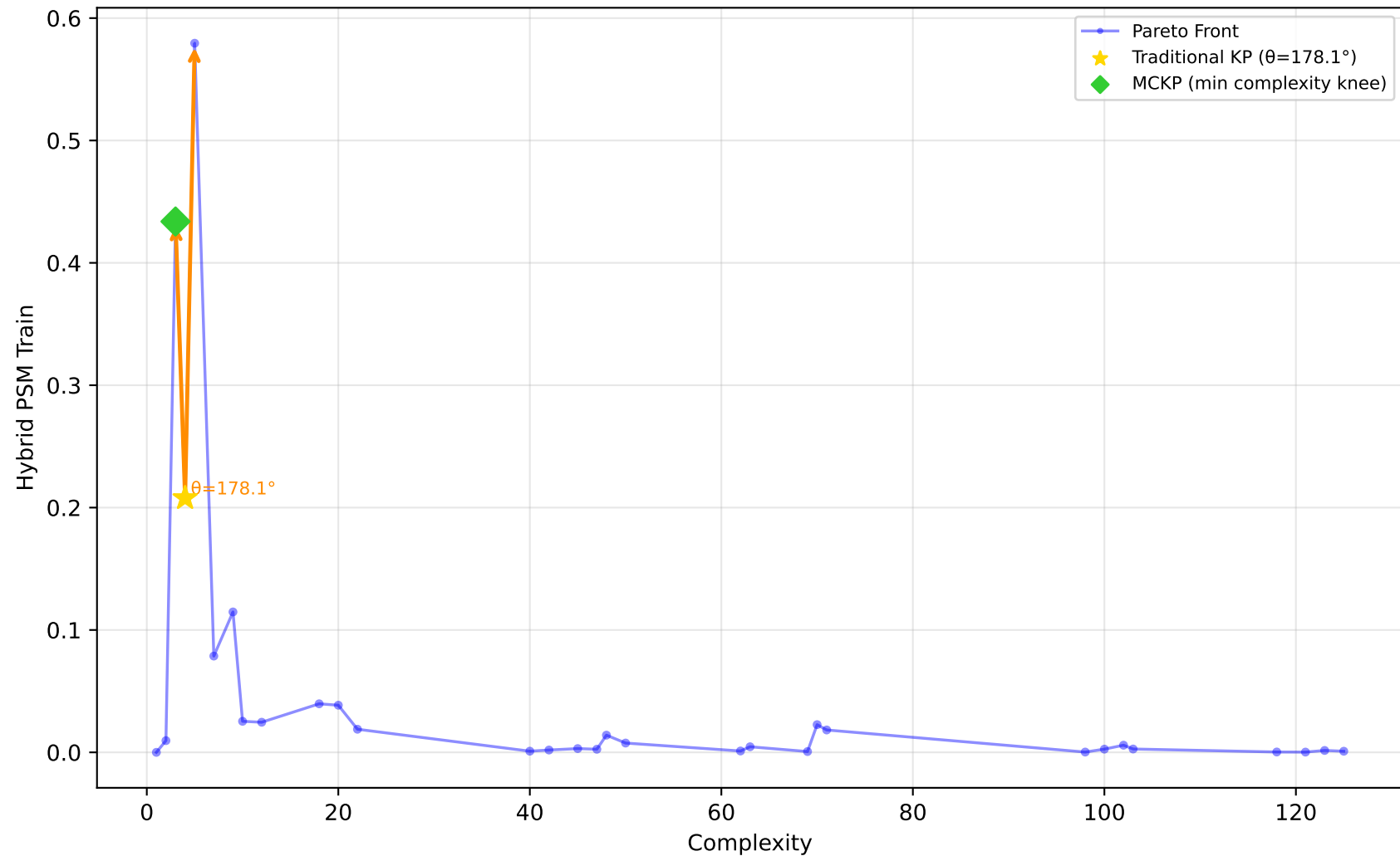
637_fri_c1_500_50 - Run 26 - SVP - Hybrid PSM Train \lambda_1=0.00, \lambda_2=0.00, \lambda_3=0.00 | Difficulty: 1.00 | Method: hmr
