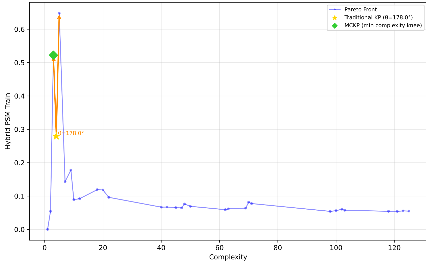
637_fri_c1_500_50 - Run 26 - SVP - Hybrid PSM Train \lambda_1=0.10, \lambda_2=0.00, \lambda_3=0.20 | Difficulty: 1.00 | Method: hmr
