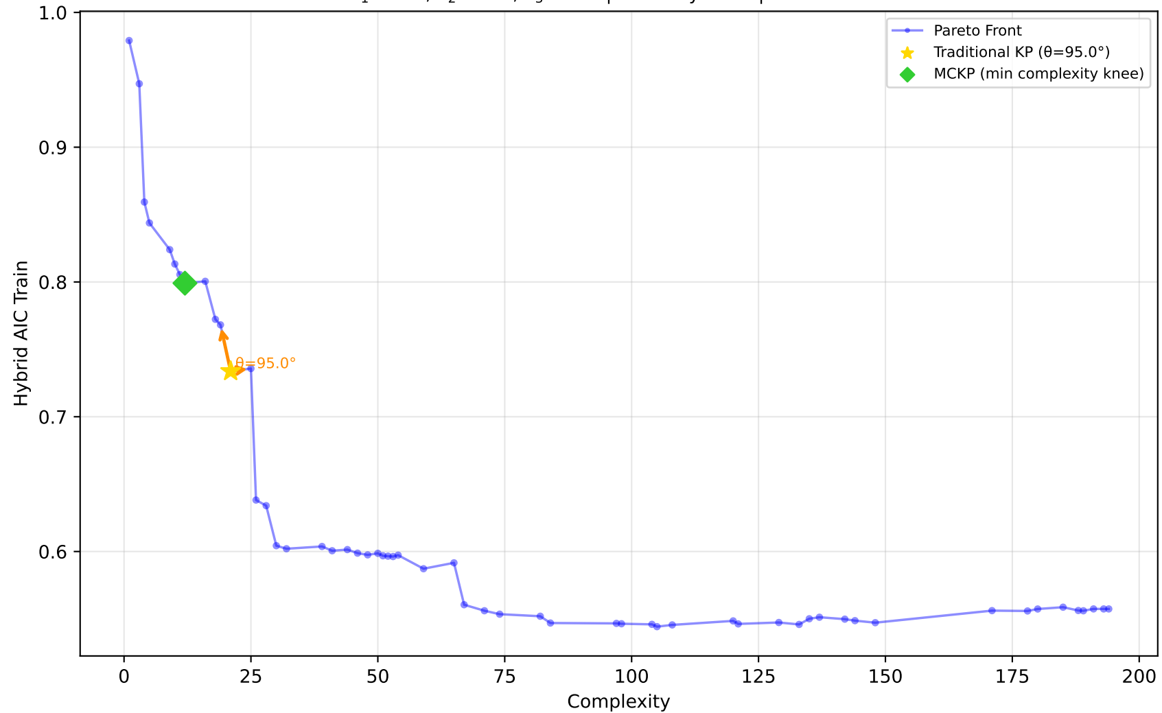
637_fri_c1_500_50 - Run 27 - MVP - Hybrid AIC Train \lambda_1=0.00, \lambda_2=0.50, \lambda_3=0.00 | Difficulty: 1.00 | Method: hmr
