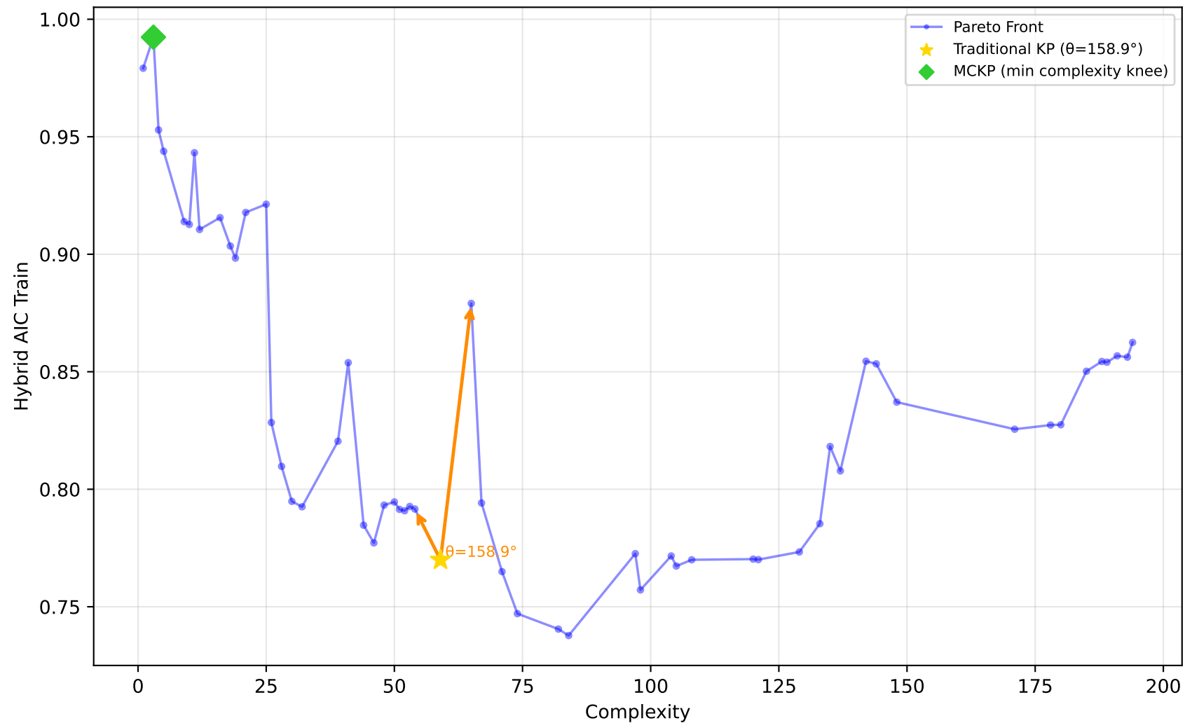
637_fri_c1_500_50 - Run 27 - MVP - Hybrid AIC Train \lambda_1=0.10 , \lambda_2=0.00 , \lambda_3=1.00 | Difficulty: 1.00 | Method: hmr
