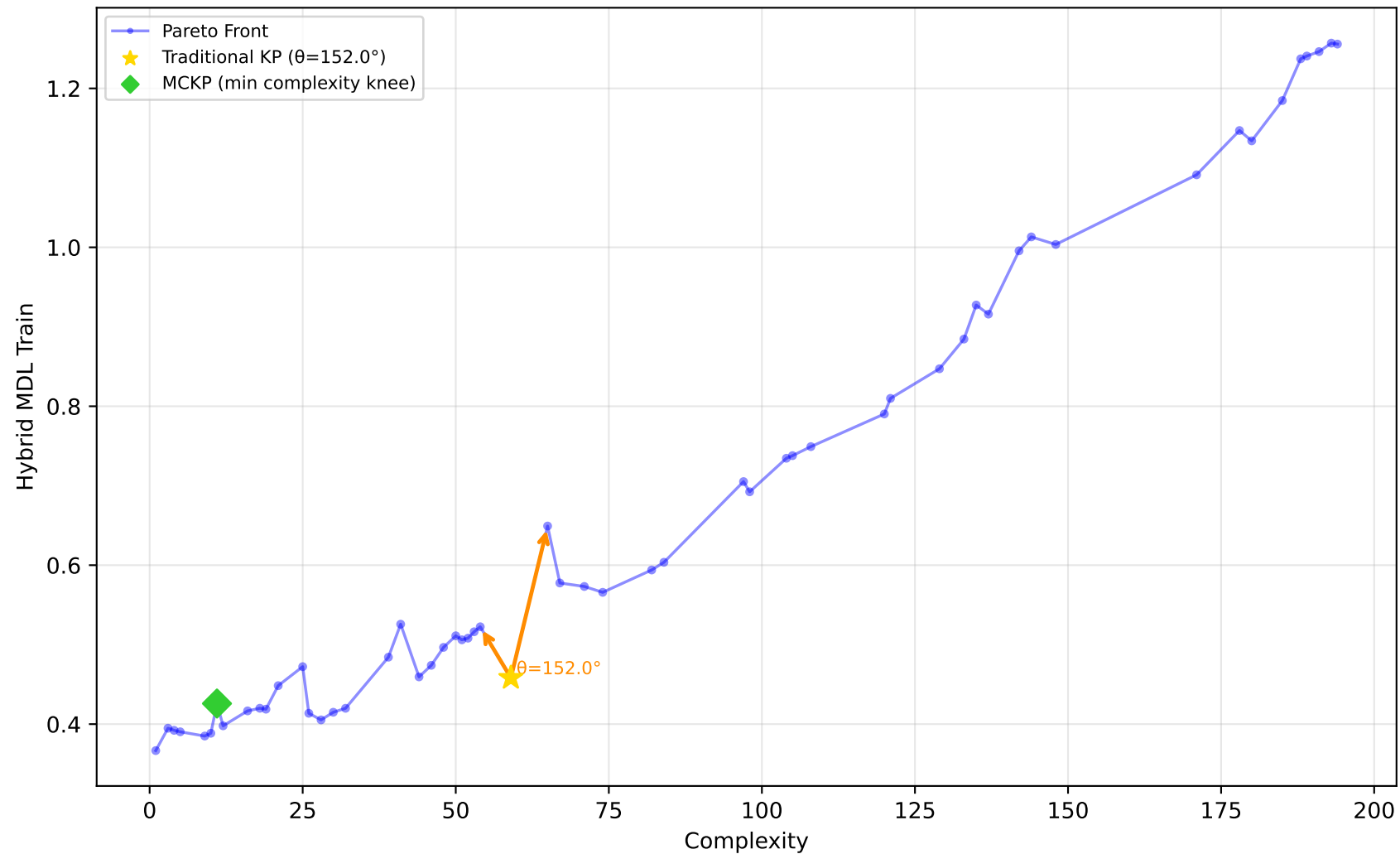
637_fri_c1_500_50 - Run 27 - MVP - Hybrid MDL Train \lambda_1=0.10, \bar{\lambda}_2=0.00, \bar{\lambda}_3=1.00 | Difficulty: 1.00 | Method: hmr
