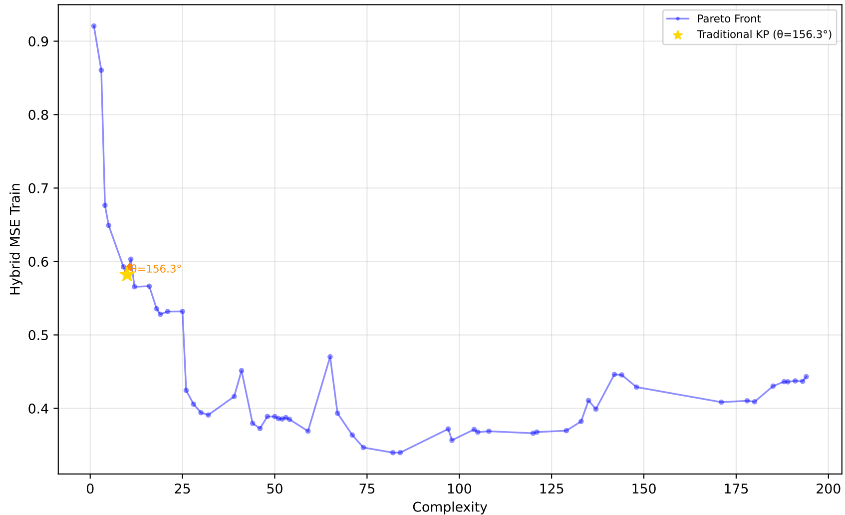
637_fri_c1_500_50 - Run 27 - MVP - Hybrid MSE Train \lambda_1=0.10, \lambda_2=0.00, \lambda_3=1.00 | Difficulty: 1.00 | Method: hmr
