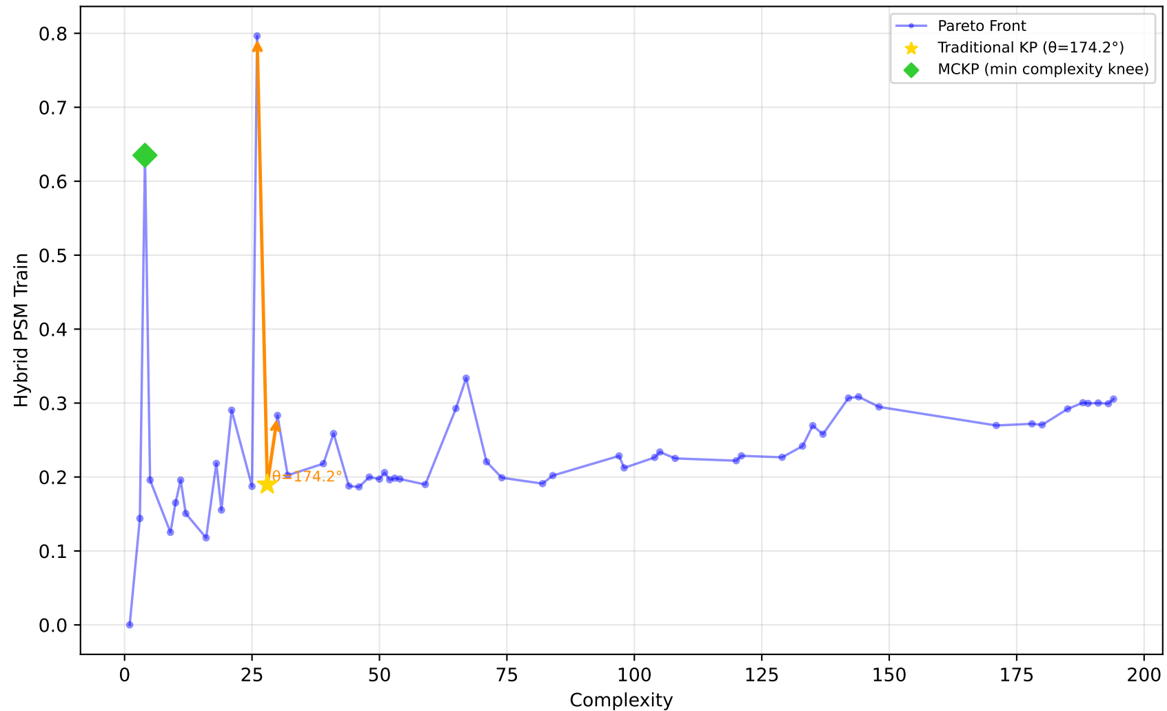
637_fri_c1_500_50 - Run 27 - MVP - Hybrid PSM Train \lambda_1=0.10, \bar{\lambda}_2=0.00, \bar{\lambda}_3=1.00 | Difficulty: 1.00 | Method: hmr
