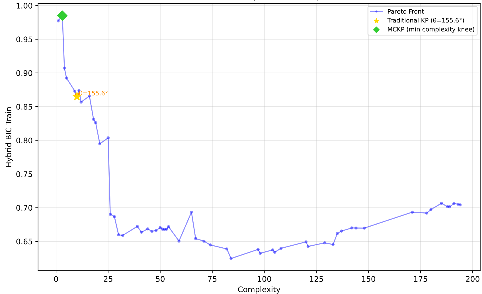
637_fri_c1_500_50 - Run 27 - SVP - Hybrid BIC Train \lambda_1=0.10 , \lambda_2=0.00 , \lambda_3=0.20 | Difficulty: 1.00 | Method: hmr
