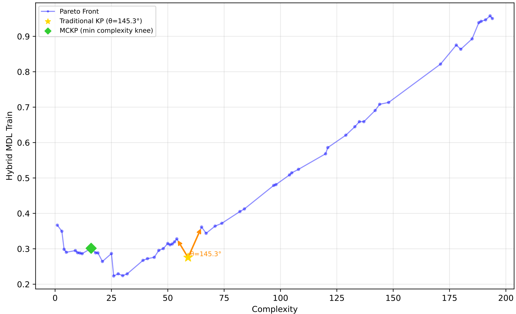
637_fri_c1_500_50 - Run 27 - SVP - Hybrid MDL Train \lambda_1=0.00, \lambda_2=0.00, \lambda_3=0.00 | Difficulty: 1.00 | Method: hmr
