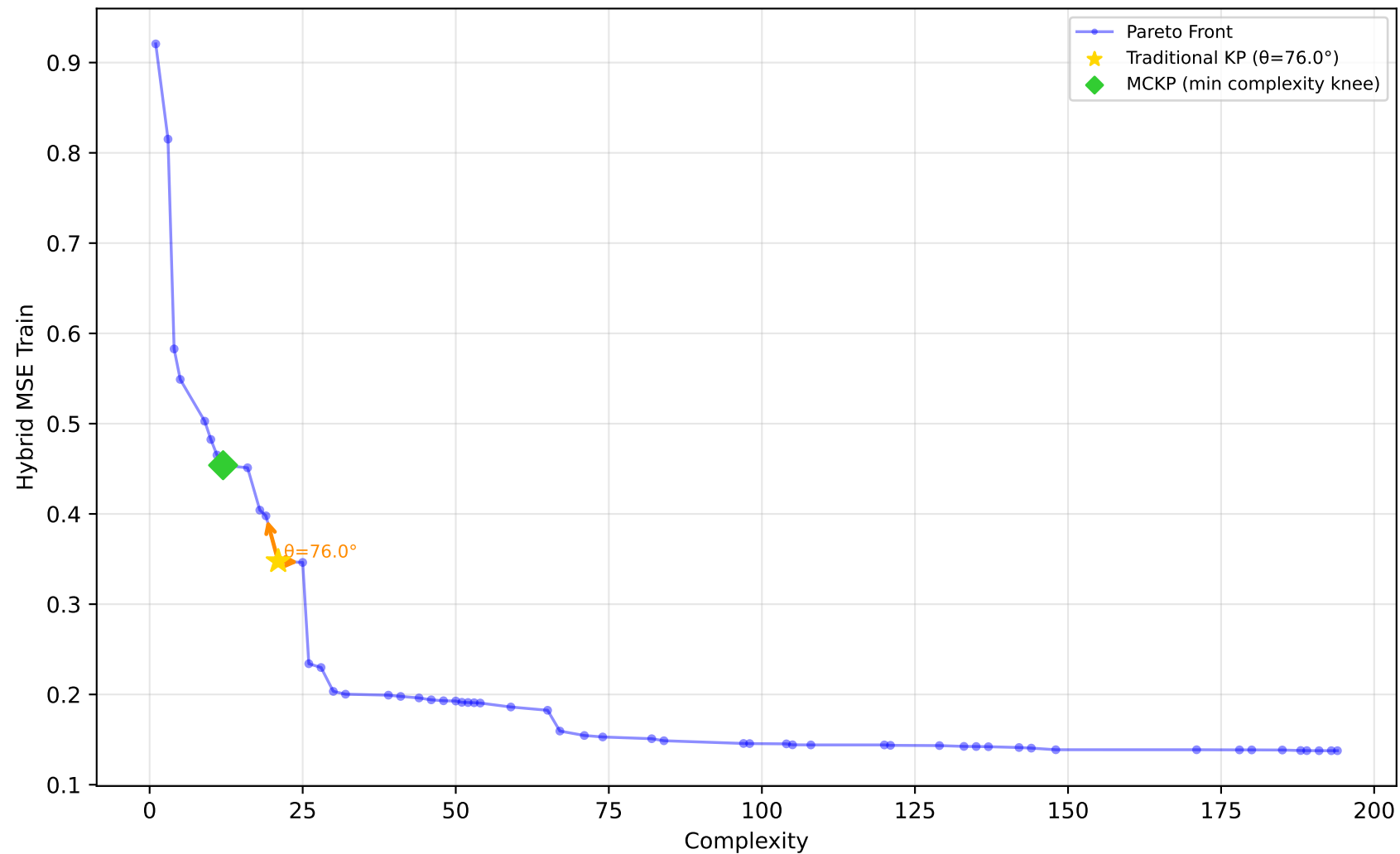
637_fri_c1_500_50 - Run 27 - SVP - Hybrid MSE Train \lambda_1=0.00, \lambda_2=0.00, \lambda_3=0.00 | Difficulty: 1.00 | Method: hmr
