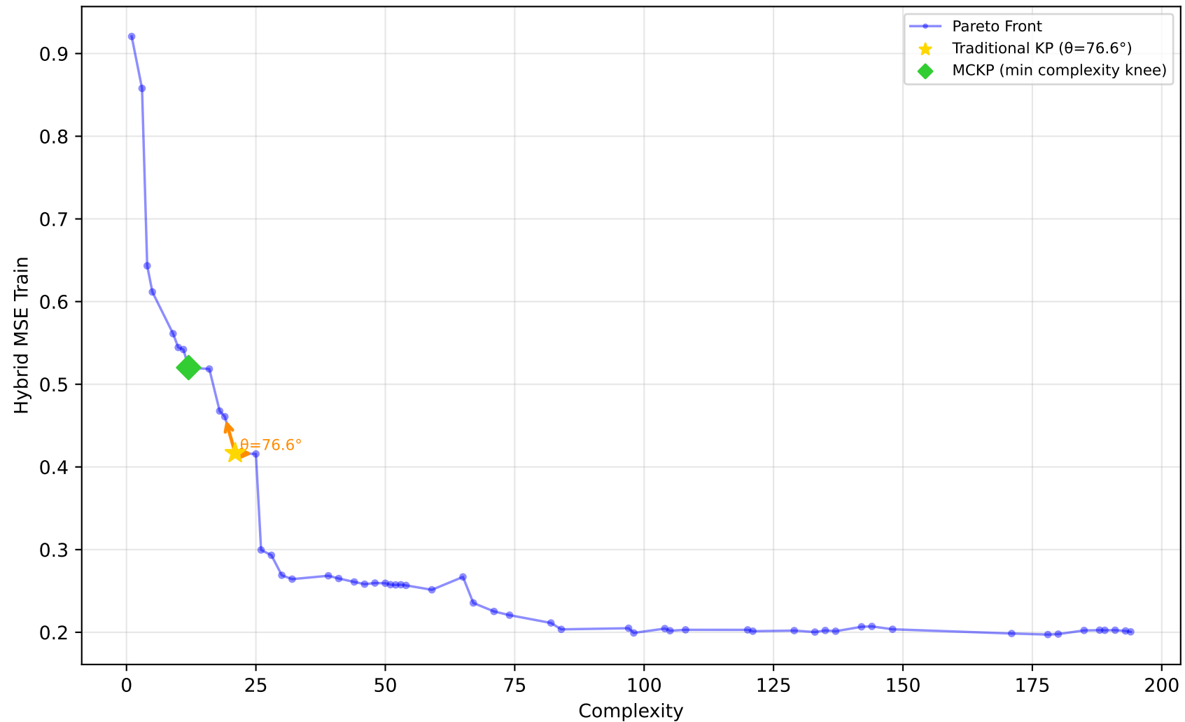
637_fri_c1_500_50 - Run 27 - SVP - Hybrid MSE Train \lambda_1=0.10, \lambda_2=0.00, \lambda_3=0.20 | Difficulty: 1.00 | Method: hmr
