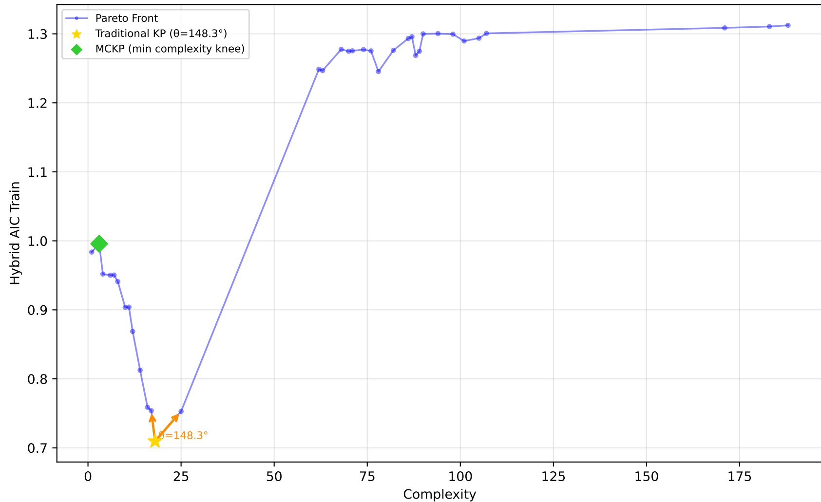
637_fri_c1_500_50 - Run 28 - MVP - Hybrid AIC Train \lambda_1=0.10, \lambda_2=0.00, \lambda_3=1.00 | Difficulty: 1.00 | Method: hmr
