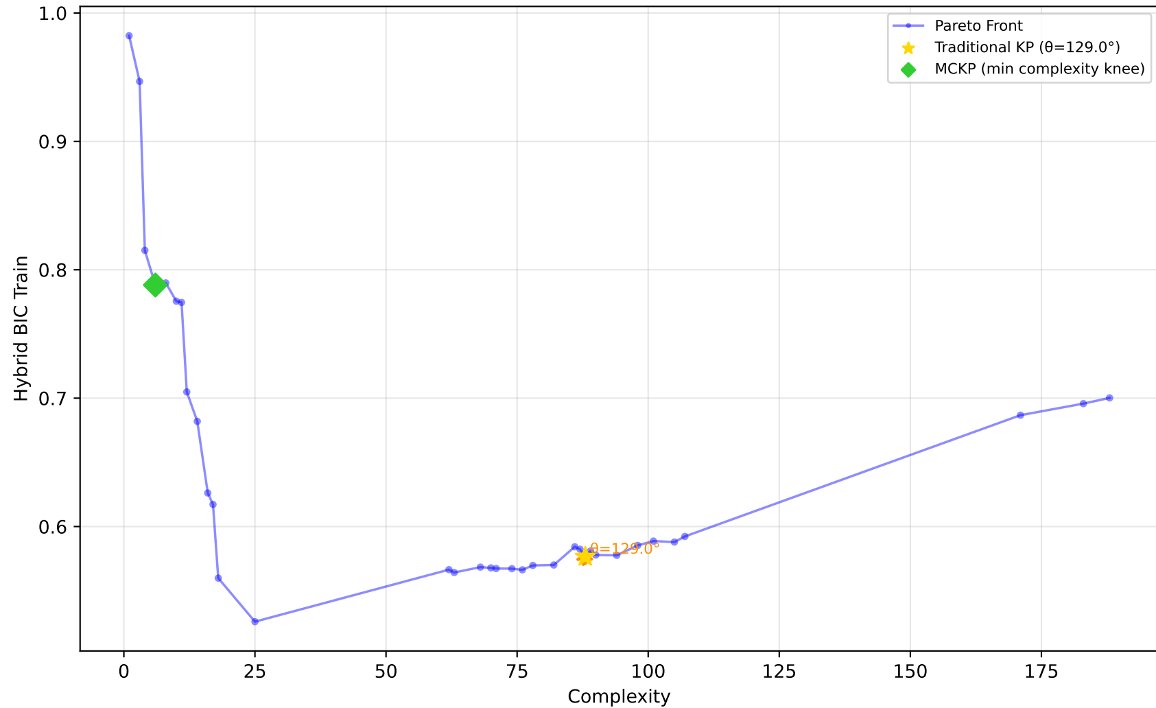
637_fri_c1_500_50 - Run 28 - MVP - Hybrid BIC Train \lambda_1=0.00, \lambda_2=0.50, \lambda_3=0.00 | Difficulty: 1.00 | Method: hmr
