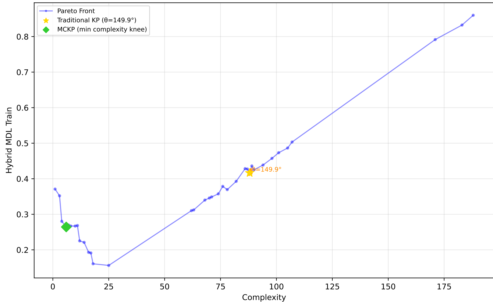
637_fri_c1_500_50 - Run 28 - MVP - Hybrid MDL Train \lambda_1=0.00, \bar{\lambda}_2=0.50, \lambda_3=0.00 | Difficulty: 1.00 | Method: hmr
