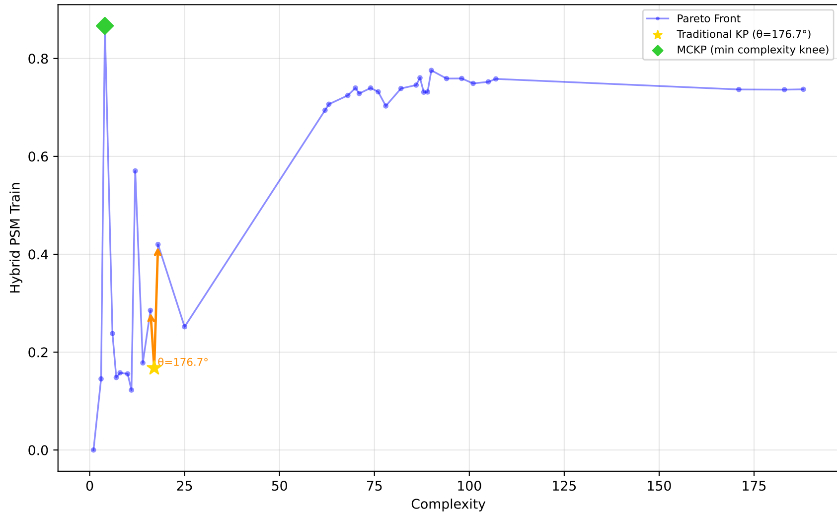
637_fri_c1_500_50 - Run 28 - MVP - Hybrid PSM Train \lambda_1=0.10, \lambda_2=0.00, \lambda_3=1.00 | Difficulty: 1.00 | Method: hmr
