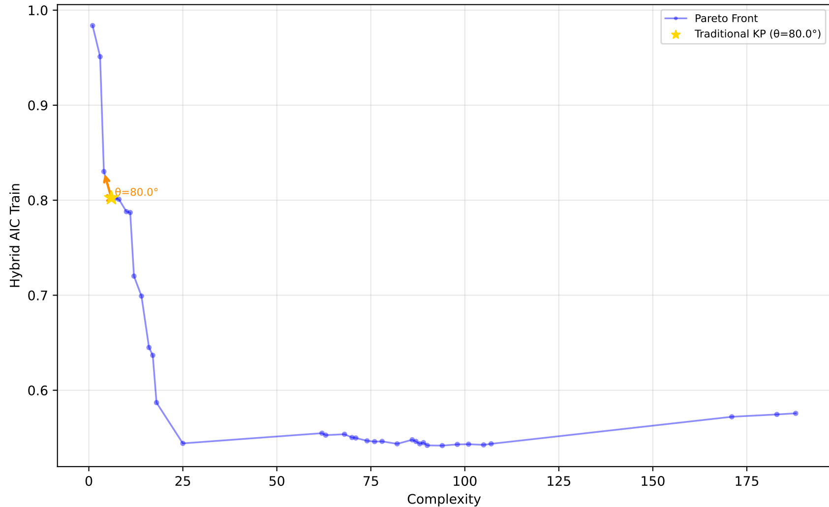
637_fri_c1_500_50 - Run 28 - SVP - Hybrid AIC Train \lambda_1=0.00, \lambda_2=0.00, \lambda_3=0.00 | Difficulty: 1.00 | Method: hmr
