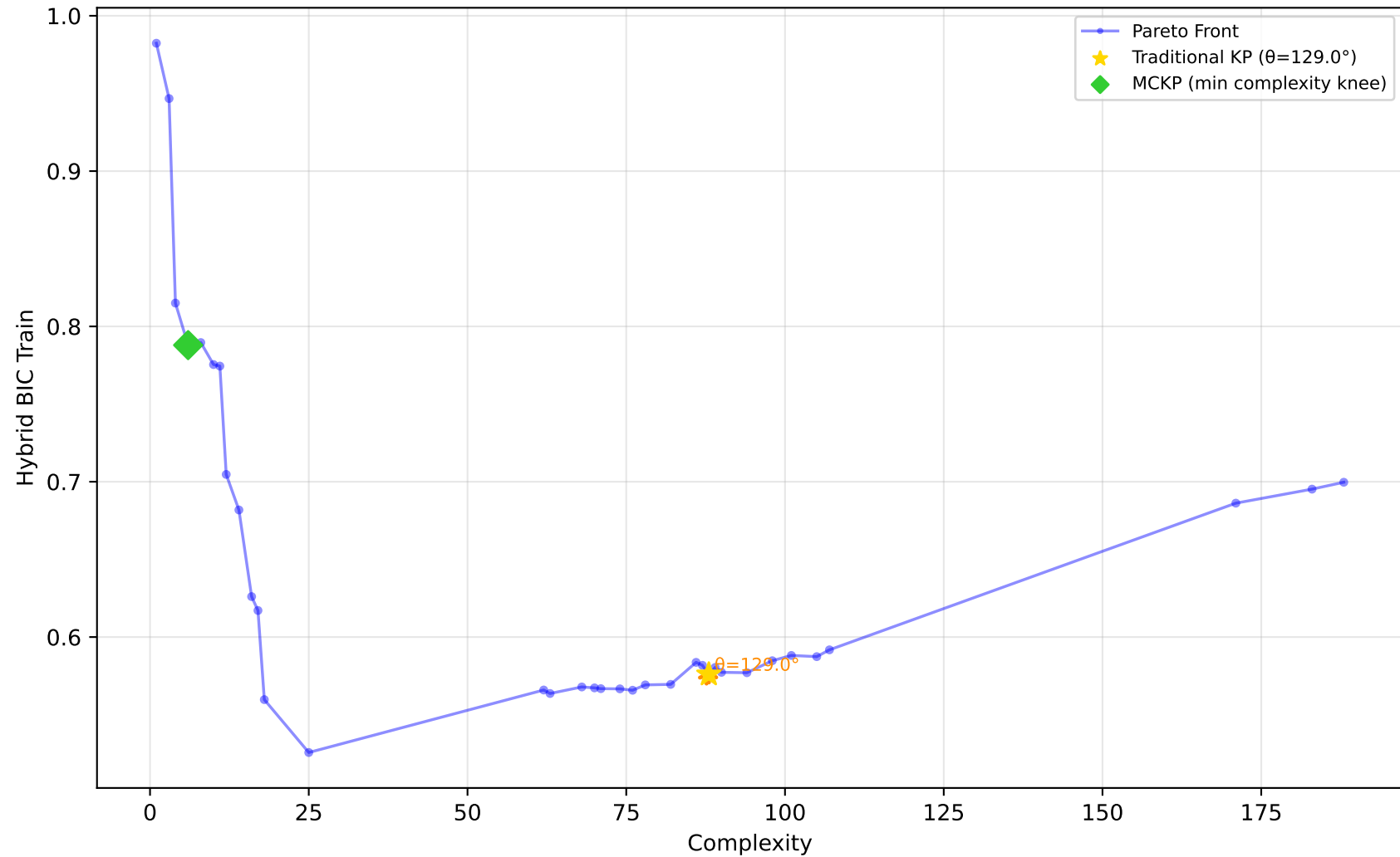
637_fri_c1_500_50 - Run 28 - SVP - Hybrid BIC Train \lambda_1=0.00, \lambda_2=0.00, \lambda_3=0.00 | Difficulty: 1.00 | Method: hmr
