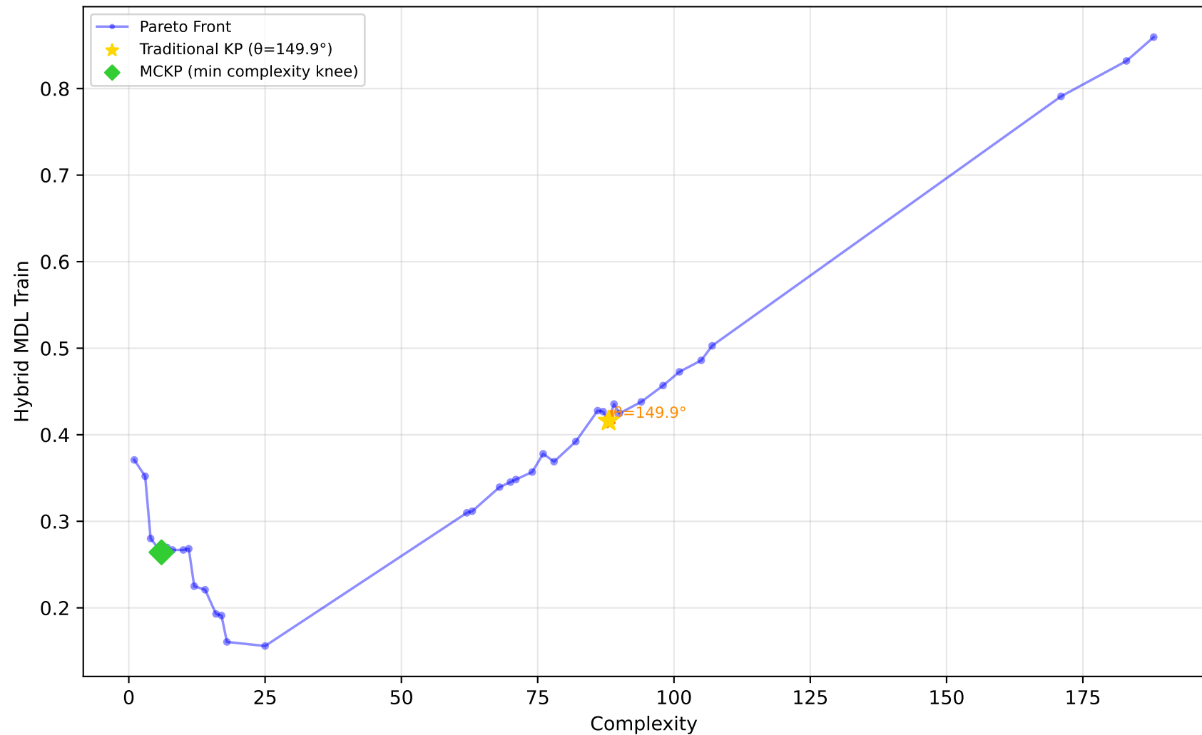
637_fri_c1_500_50 - Run 28 - SVP - Hybrid MDL Train \lambda_1=0.00, \lambda_2=0.00, \lambda_3=0.00 | Difficulty: 1.00 | Method: hmr
