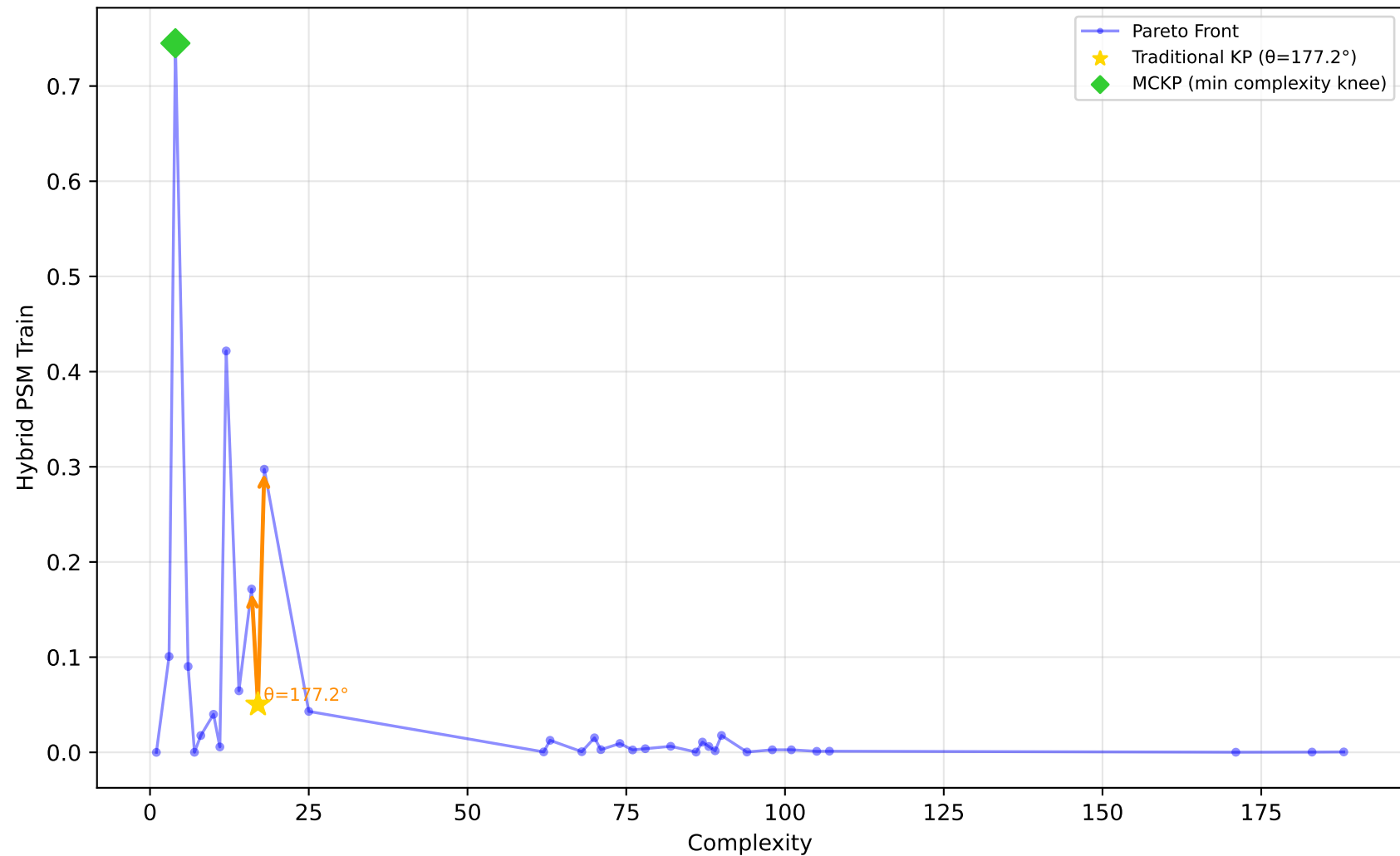
637_fri_c1_500_50 - Run 28 - SVP - Hybrid PSM Train \lambda_1=0.00, \lambda_2=0.00, \lambda_3=0.00 | Difficulty: 1.00 | Method: hmr
