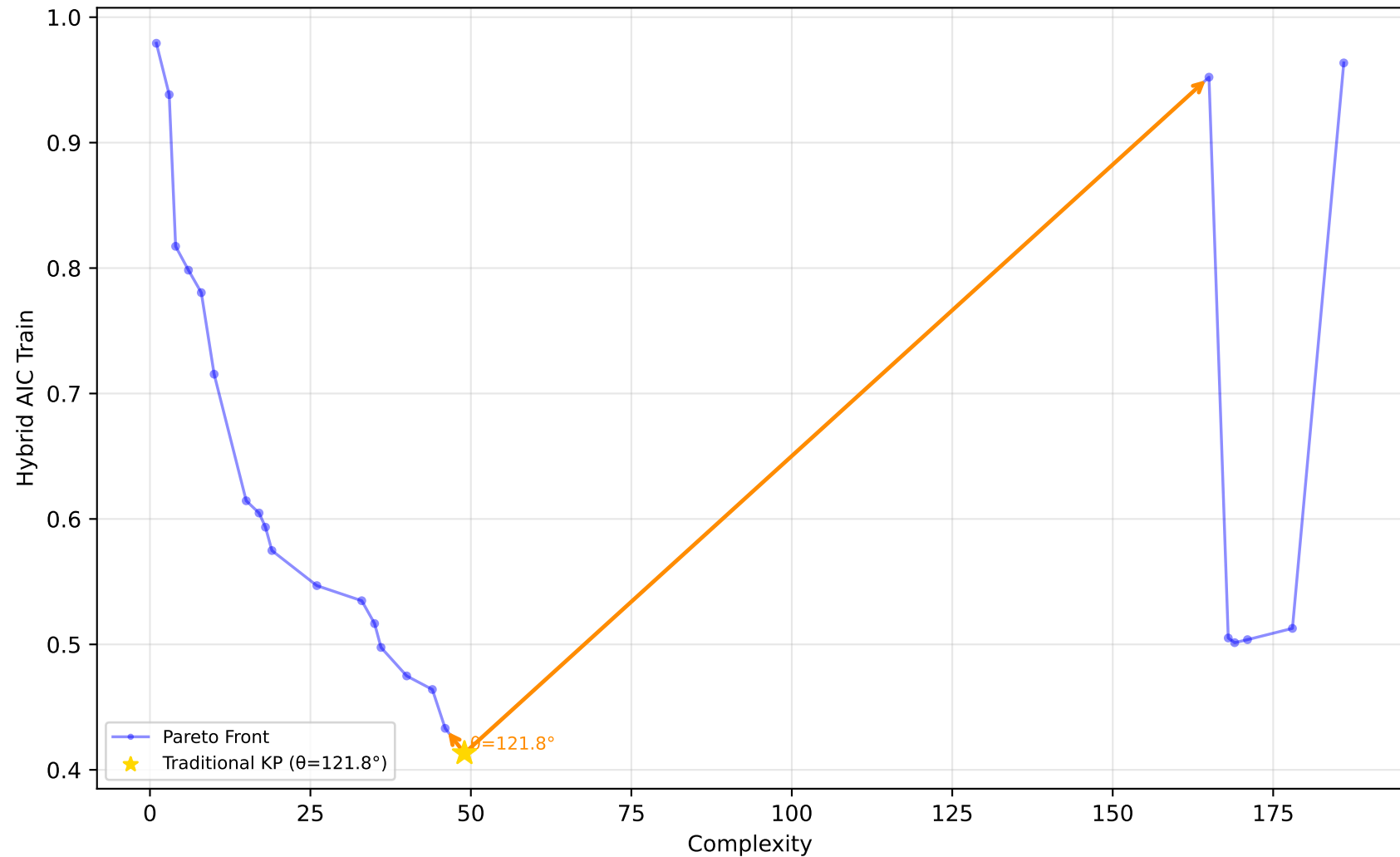
637_fri_c1_500_50 - Run 29 - MVP - Hybrid AIC Train \lambda_1=0.00, \lambda_2=0.50, \lambda_3=0.00 | Difficulty: 1.00 | Method: hmr
