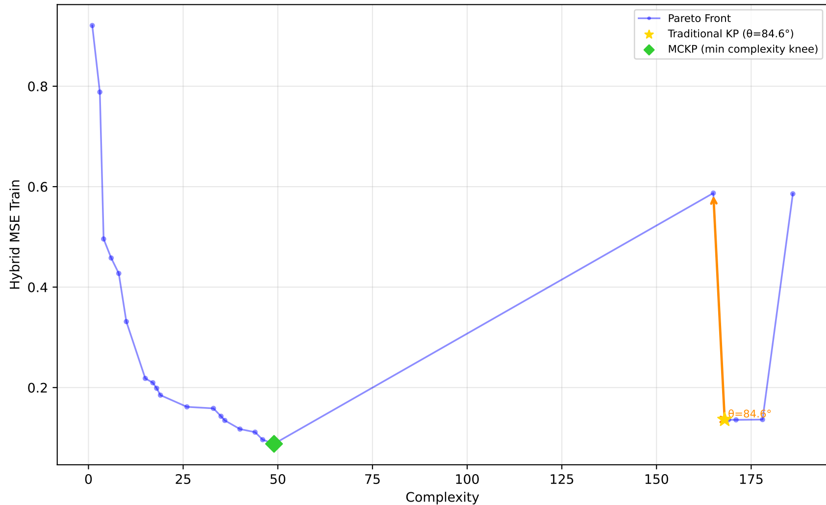
637_fri_c1_500_50 - Run 29 - MVP - Hybrid MSE Train \lambda_1=0.00, \bar{\lambda}_2=0.50, \lambda_3=0.00 | Difficulty: 1.00 | Method: hmr
