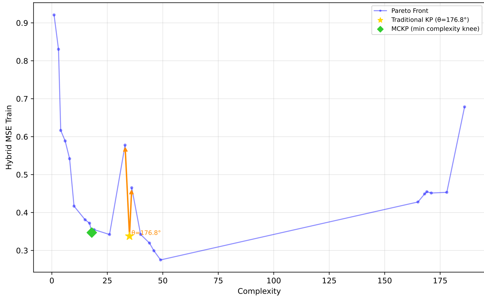
637_fri_c1_500_50 - Run 29 - MVP - Hybrid MSE Train \lambda_1=0.10, \bar{\lambda}_2=0.00, \bar{\lambda}_3=1.00 | Difficulty: 1.00 | Method: hmr
