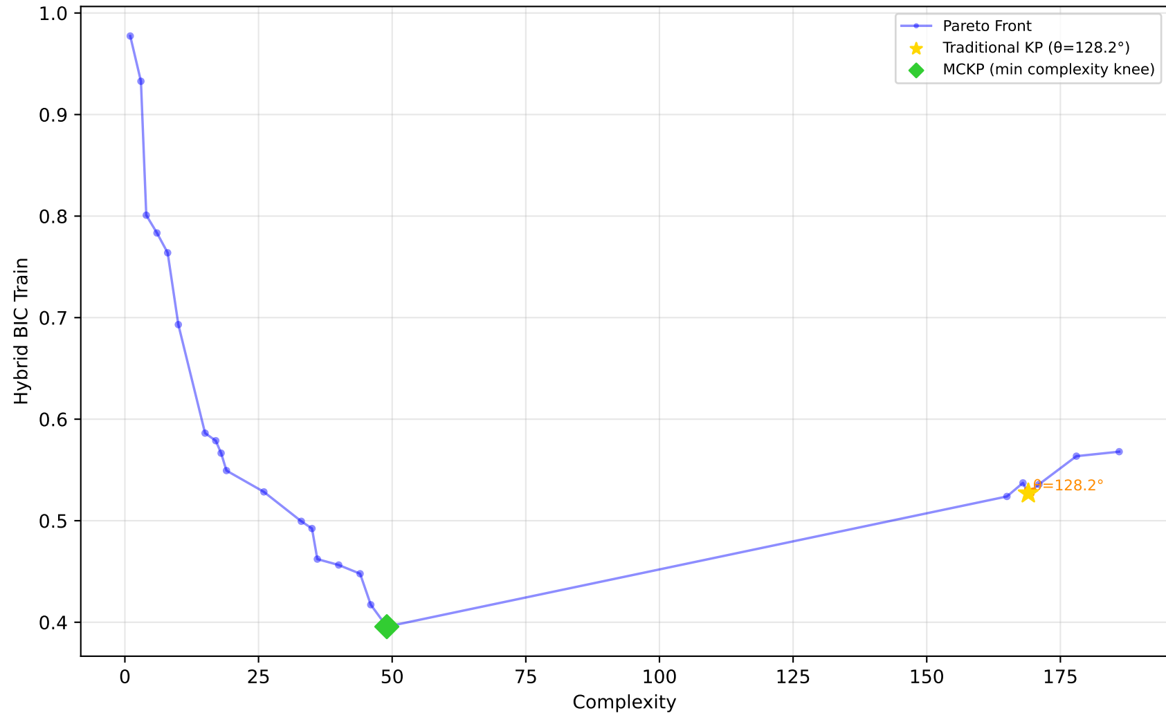
637_fri_c1_500_50 - Run 29 - SVP - Hybrid BIC Train \lambda_1=0.00, \lambda_2=0.00, \lambda_3=0.00 | Difficulty: 1.00 | Method: hmr
