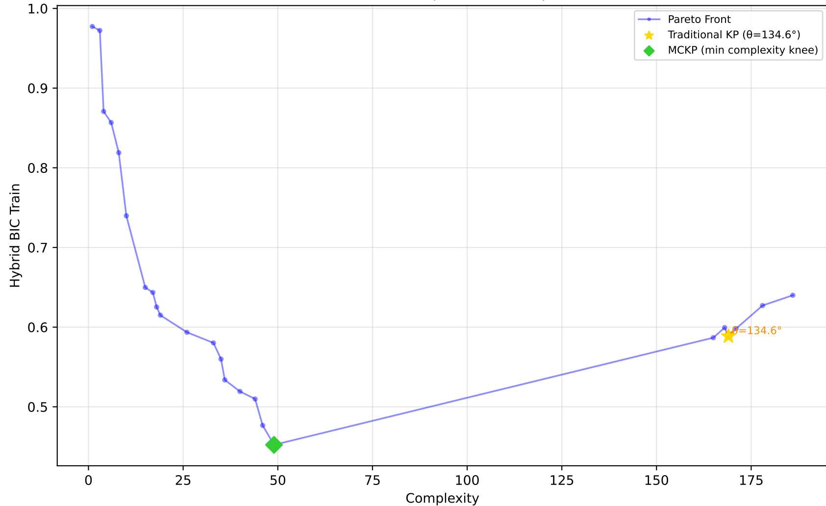
637_fri_c1_500_50 - Run 29 - SVP - Hybrid BIC Train \lambda_1=0.10, \lambda_2=0.00, \lambda_3=0.20 | Difficulty: 1.00 | Method: hmr
