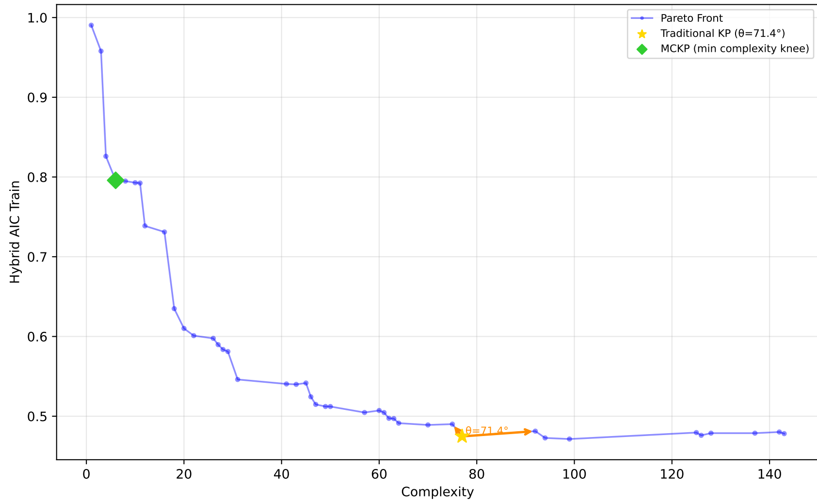
637_fri_c1_500_50 - Run 2 - MVP - Hybrid AIC Train \lambda_1=0.00, \lambda_2=0.50, \lambda_3=0.00 | Difficulty: 1.00 | Method: hmr
