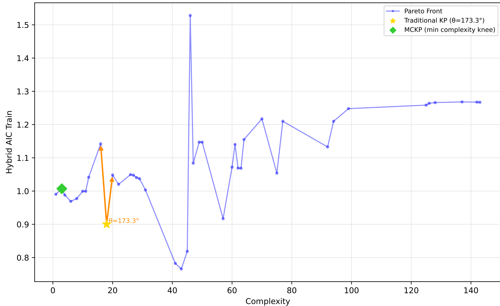
637_fri_c1_500_50 - Run 2 - MVP - Hybrid AIC Train \lambda_1=0.10, \lambda_2=0.00, \lambda_3=1.00 | Difficulty: 1.00 | Method: hmr
