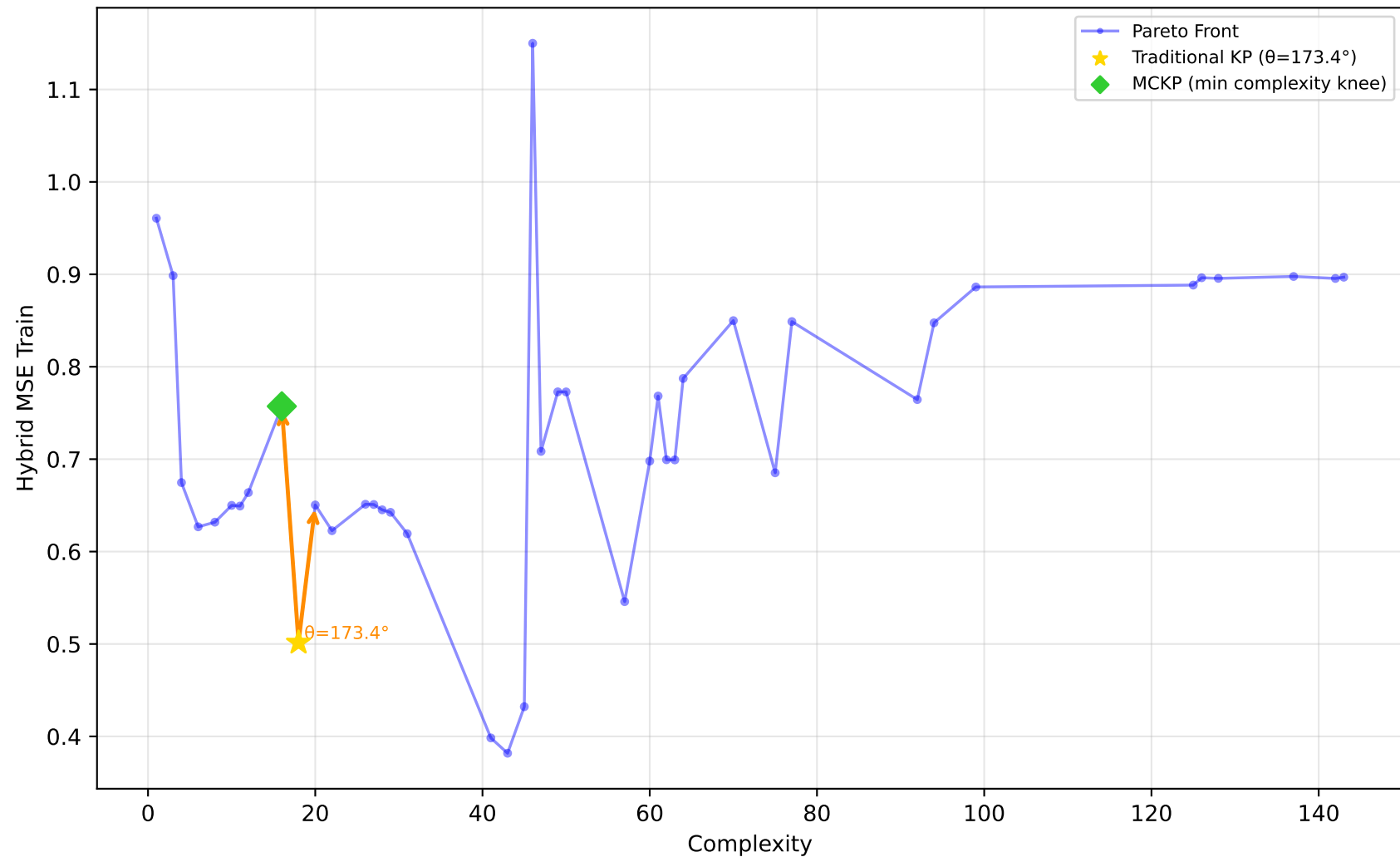
637_fri_c1_500_50 - Run 2 - MVP - Hybrid MSE Train \lambda_1=0.10, \lambda_2=0.00, \lambda_3=1.00 | Difficulty: 1.00 | Method: hmr
