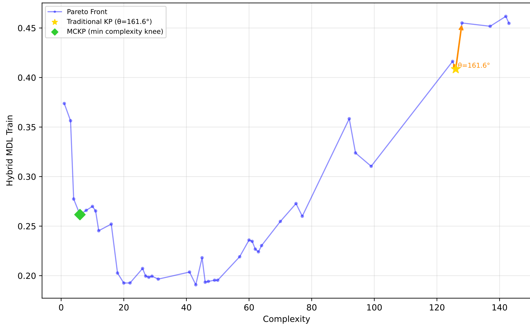
637_fri_c1_500_50 - Run 2 - SVP - Hybrid MDL Train \lambda_1=0.00, \lambda_2=0.00, \lambda_3=0.00 | Difficulty: 1.00 | Method: hmr
