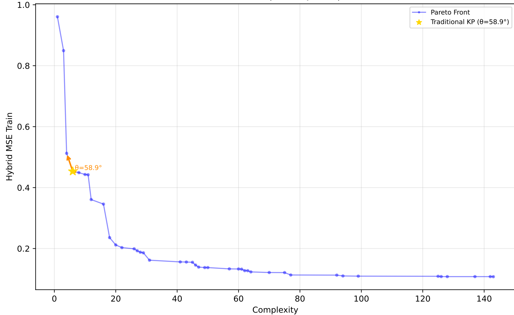
637_fri_c1_500_50 - Run 2 - SVP - Hybrid MSE Train \lambda_1=0.00, \lambda_2=0.00, \lambda_3=0.00 | Difficulty: 1.00 | Method: hmr
